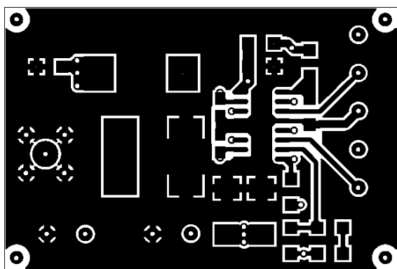
Figure 6. Top Layer
