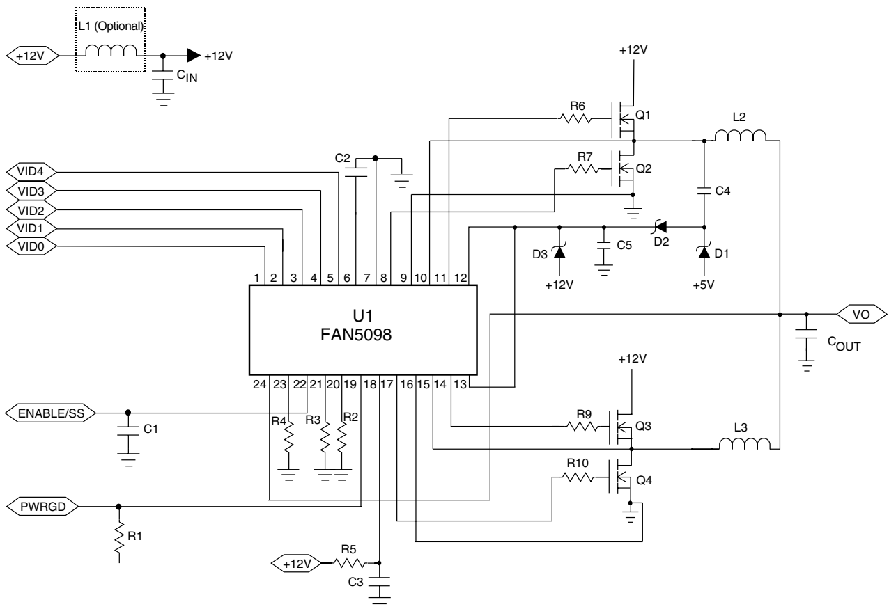
Figure 1. Application Circuit for 31A AMD Hammer Desktop Application (500 KHz each phase)
