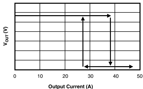
Figure 3. FAN5056 Short Circuit Characteristic
