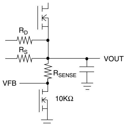
Figure 6. Using VADJ to Generate VTT
