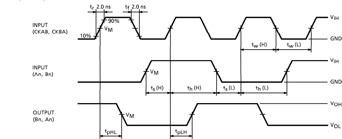
Fig.3 t_{pLH}, t_{pHL}, t_w, t_s, t_h
