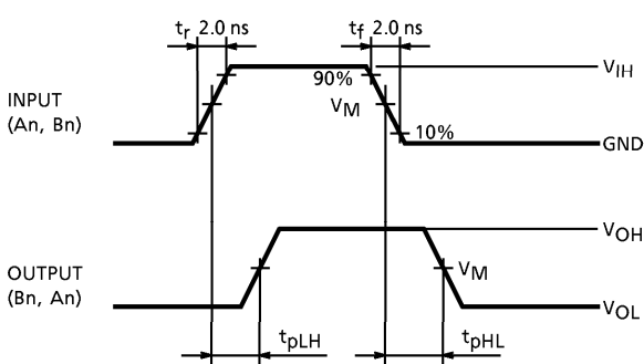
AC WAVEFORM Fig.2 t_{pLH}, t_{pHL}
