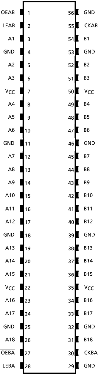
(TOP VIEW)
