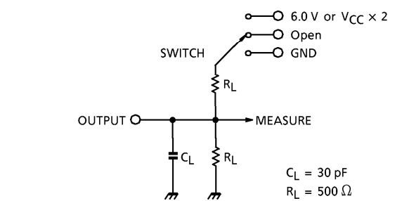
TEST CIRCUIT Fig.1
