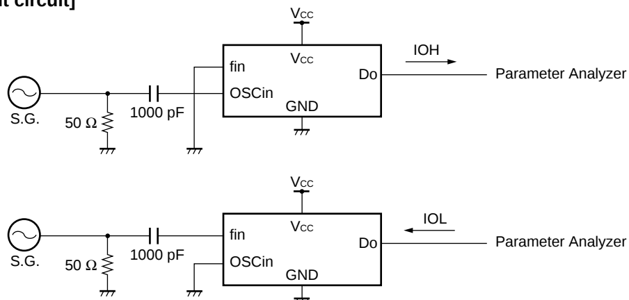
[Measurement circuit]
