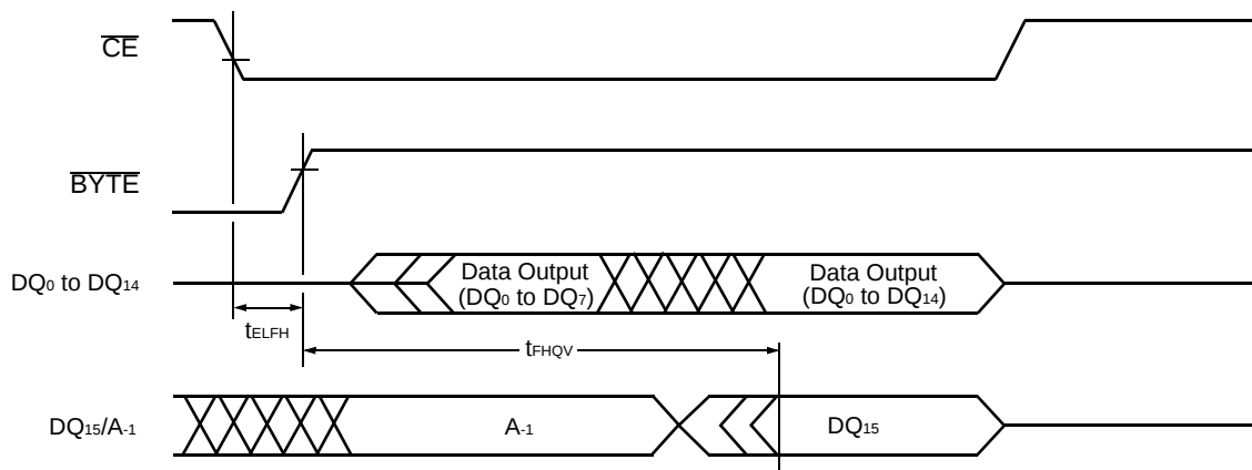
Figure 10 Timing Diagram for Word Mode Configuration
