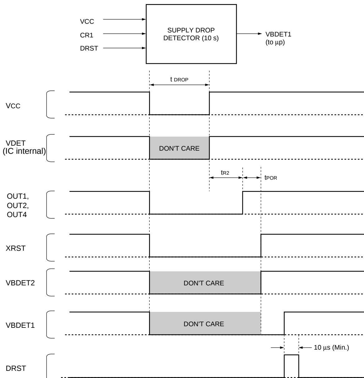
Figure 9. Power Supply Drop Detector 2 (Initial power supply detector/Power supply drop detector) a) t > 10 s
