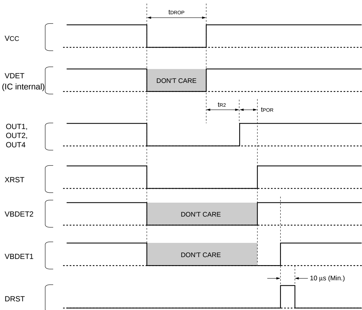
Figure 9. Power Supply Drop Detector 2 (Initial power supply detector/Power supply drop detector) b) 1.5 \text{ s} < t < 10 \text{ s}
