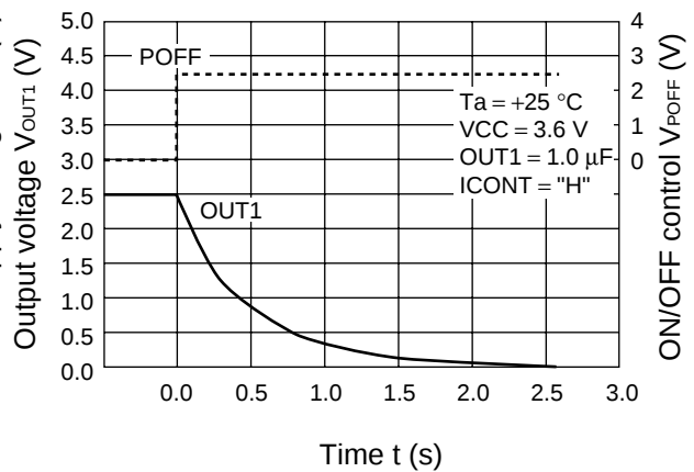
Output voltage falling waveforms (REG1 ON/OFF Control)
