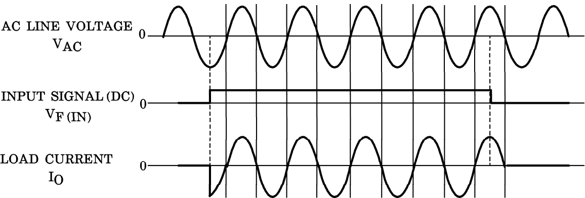
Fig.1 SWITCHING WAVEFORM
