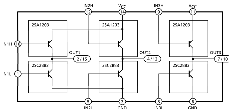
SSOP16-P-225-1.00A
