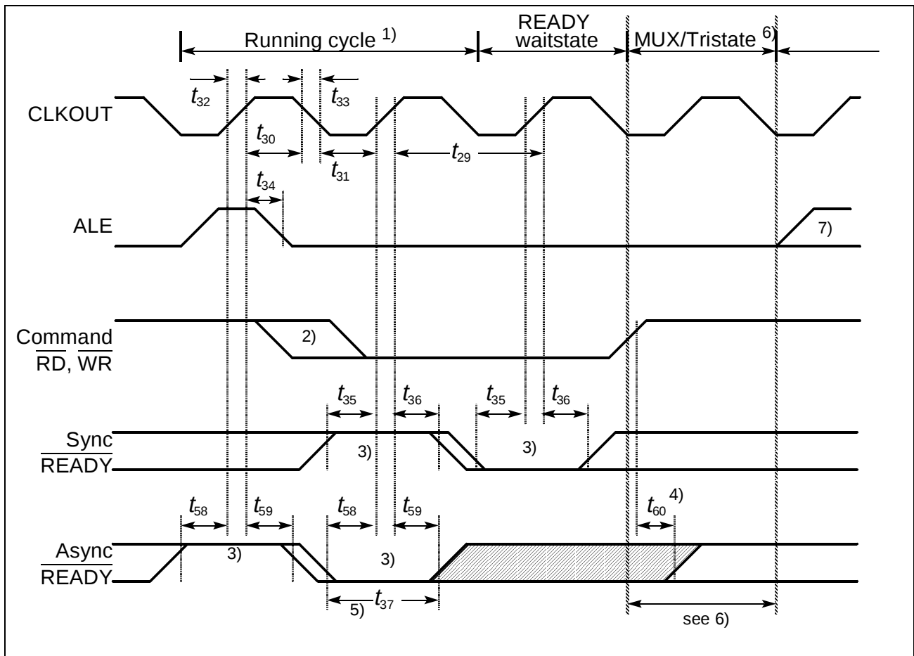
Figure 20 CLKOUT and READY
