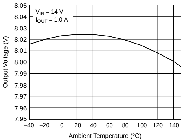
Figure 2. Regulator 1 Output Voltage
