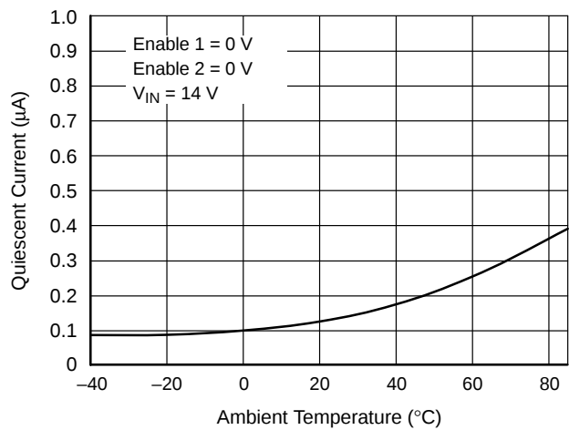
Figure 9. Quiescent Current
