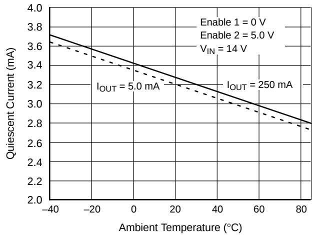
Figure 11. Regulator 2 Quiescent Current
