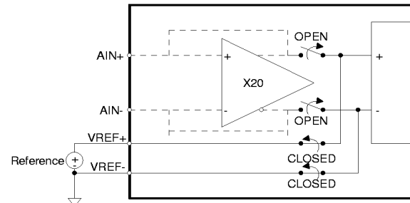
Figure 12. Self Calibration of Gain (All Ranges).
