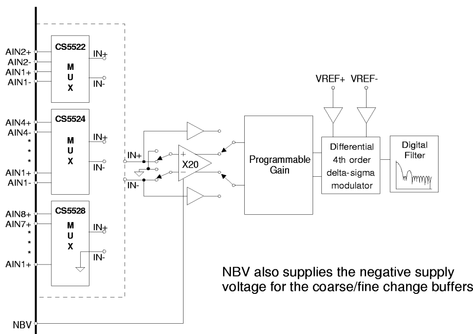
Figure 7. Multiplexer Configuration
