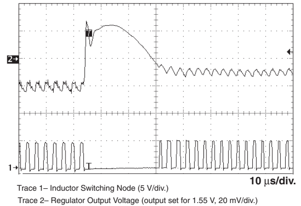
Figure 11. CS5161/5161H Pentium® III Converter Output Voltage Response to a 12 to 0 A Load Decrease
