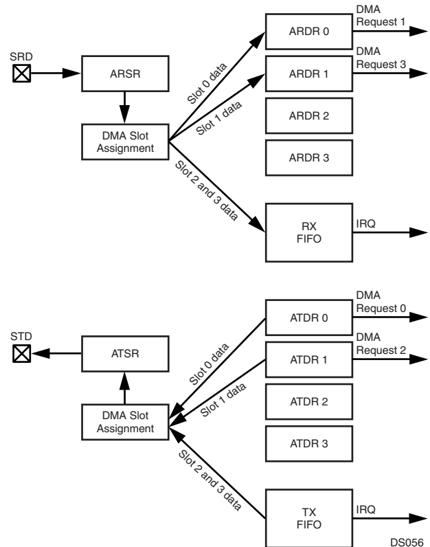
Figure 55. IRQ/DMA Support in Network Mode
