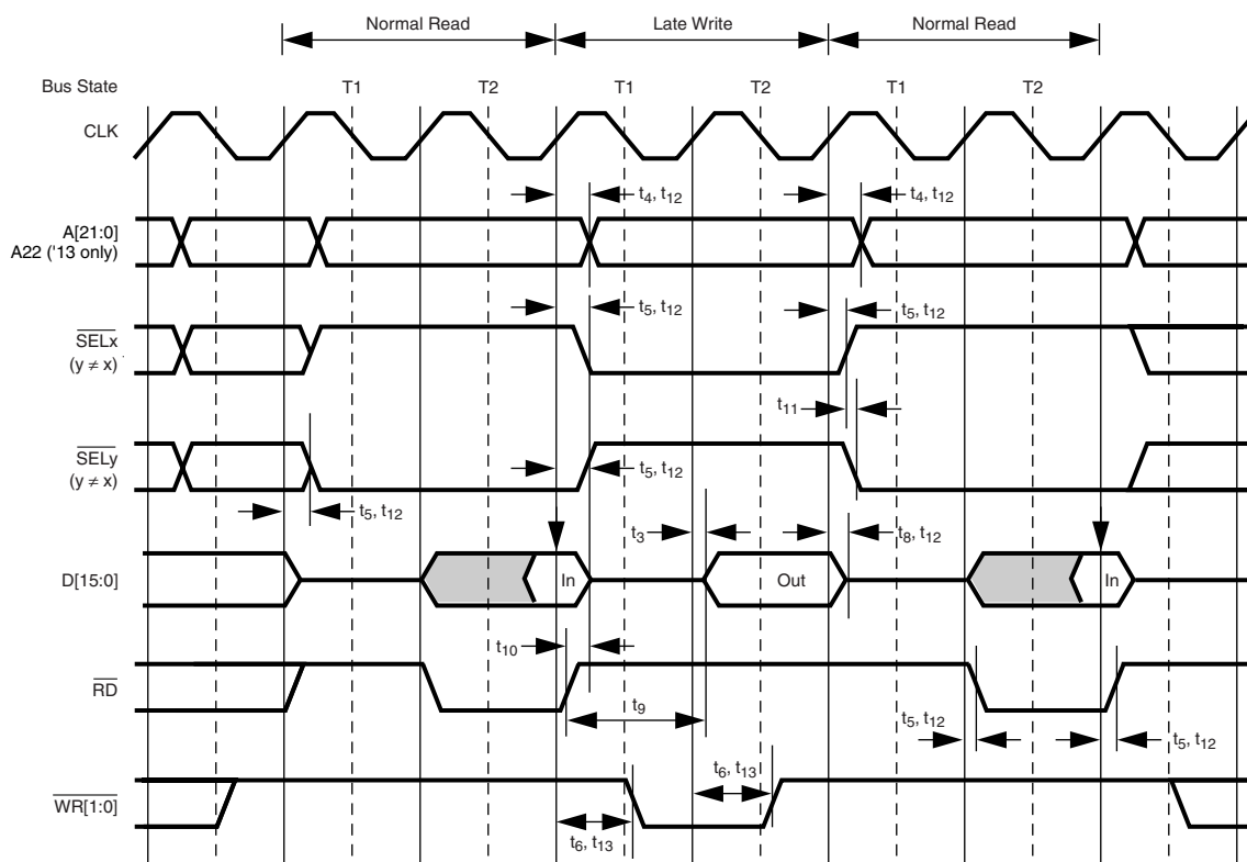
Figure 119. Late Write Between Normal Read Cycles (No Wait States)
