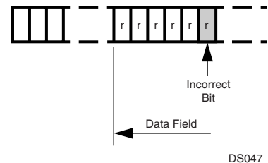
Figure 50. EBID Example
