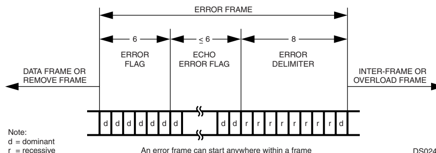
Figure 27. Error Frame
