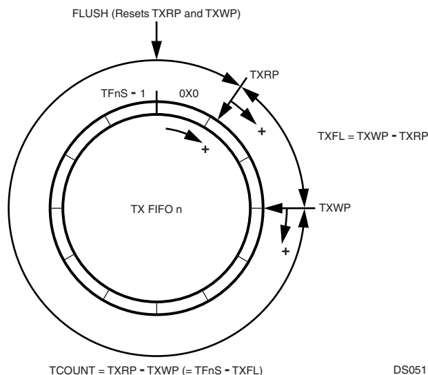
Figure 18. Transmit FIFO Operation
