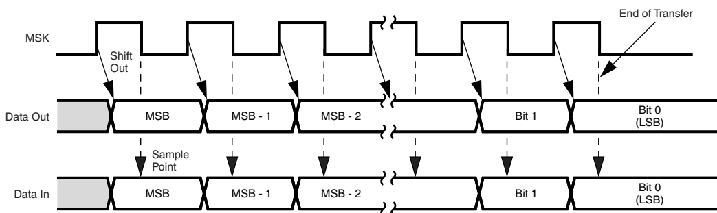
Figure 74. Alternate Mode (SCIDL = 0)
