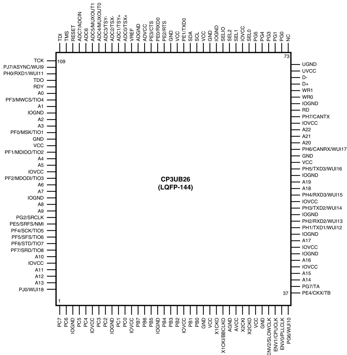
Figure 124. CP3UB26 in the LQFP-144 Package (Top View)
