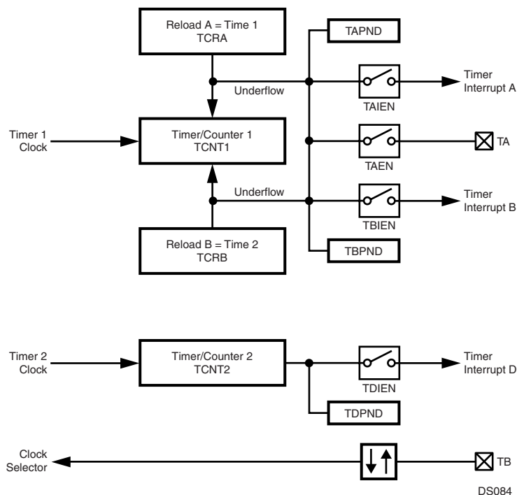
Figure 87. Processor-Independent PWM Mode
