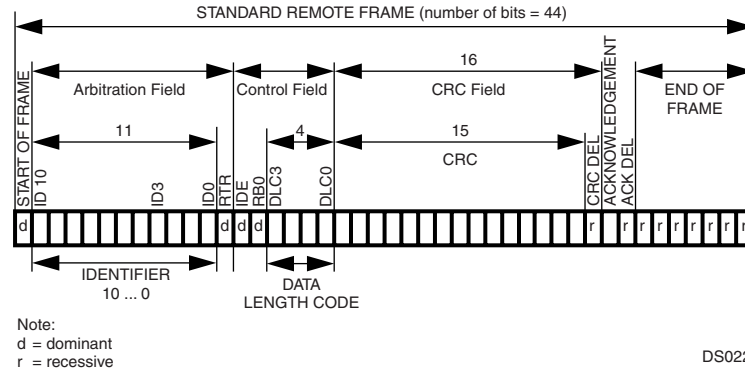
Figure 25. Standard Remote Frame
