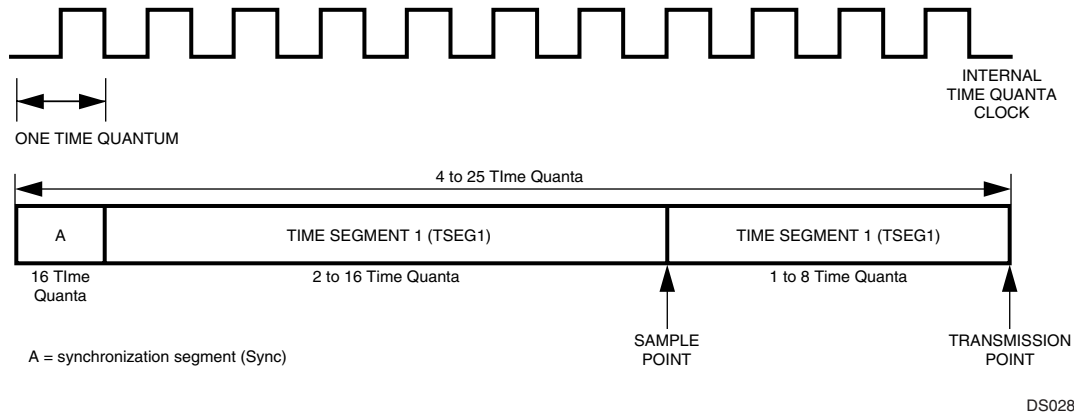
Figure 31. Bit Timing
