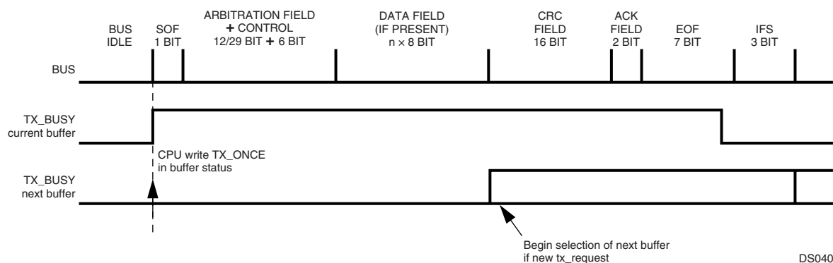
Figure 43. Data Transmission
