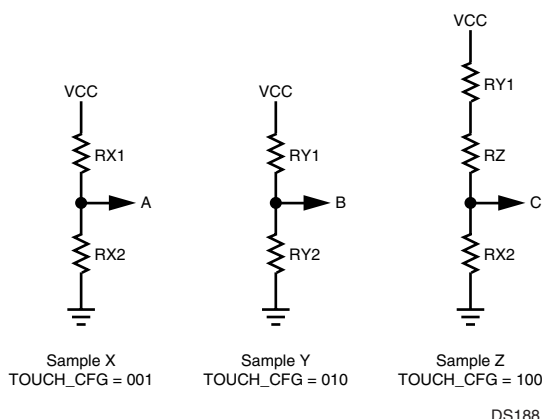
Figure 14. Touchscreen Driver Modes
