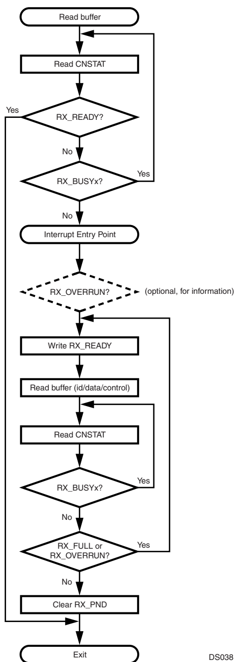
Figure 41. Buffer Read Routine (BUFFLOCK Disabled)
