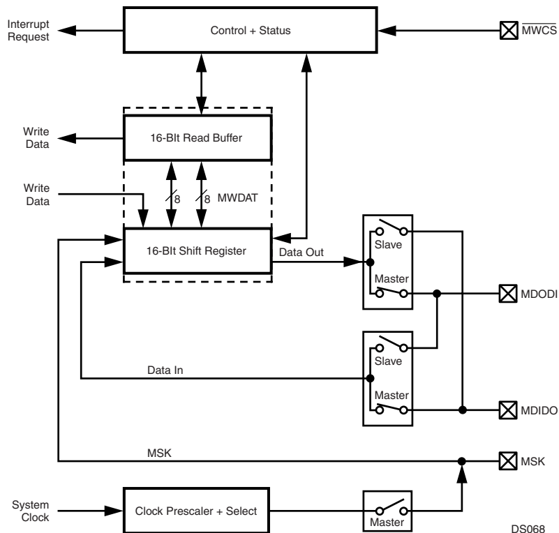
Figure 71. Microwire Block Diagram
