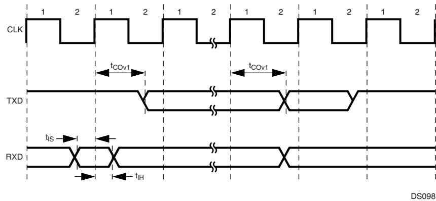
Figure 101. UART Asynchronous Mode Timing
