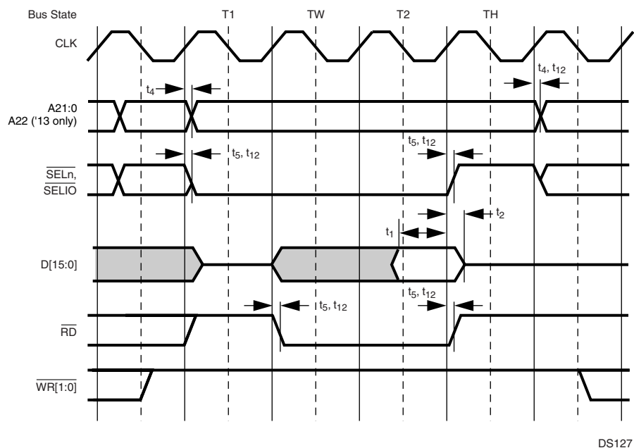
Figure 121. Normal Read Cycle (Wait Cycle Followed by Hold Cycle)
