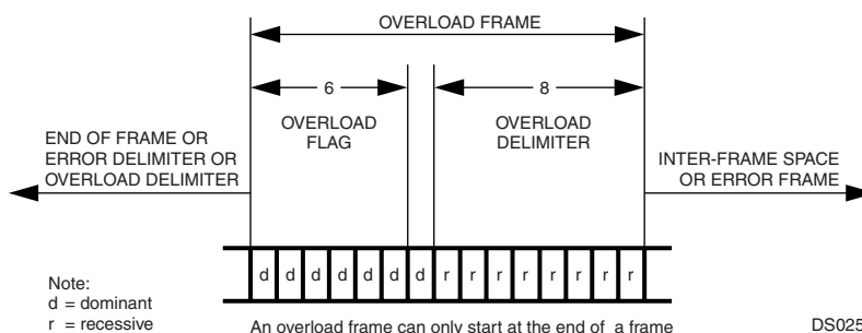
Figure 28. Overload Frame
