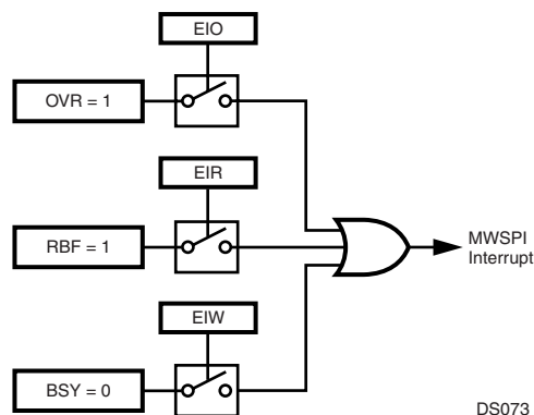
Figure 76. MWSPi Interrupts
