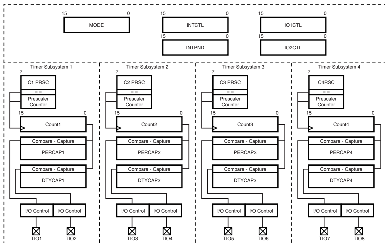
Figure 91. Versatile Timer Unit Block Diagram
