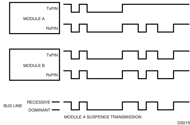
Figure 22. CAN Message Arbitration
