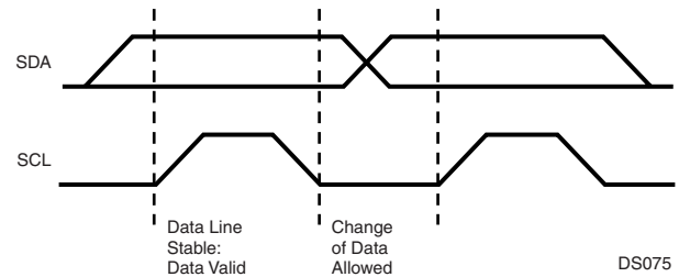
Figure 78. Bit Transfer
