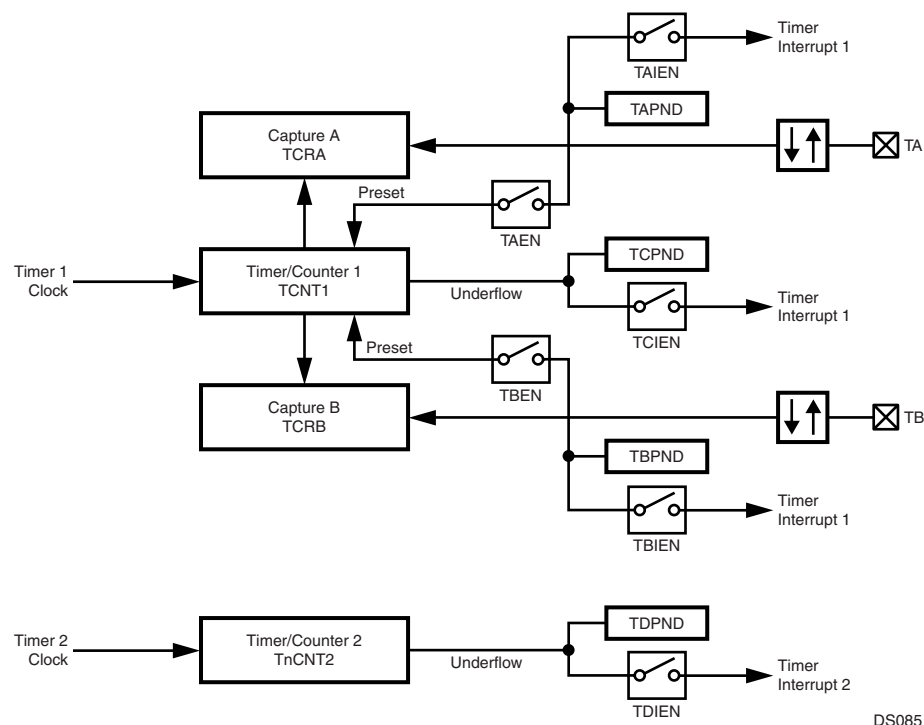
Figure 88. Dual-Input Capture Mode
