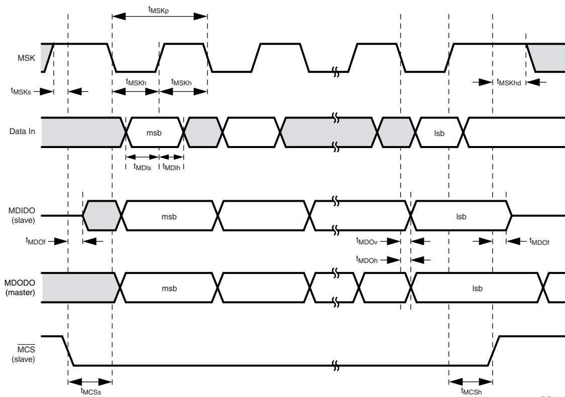
Figure 108. Microwire Transaction Timing, Normal Mode, SCIDL = 1
