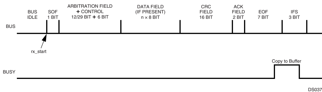
Figure 40. Receive Timing
