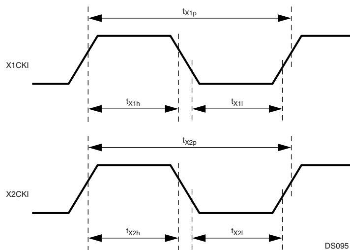
Figure 97. Clock Timing
