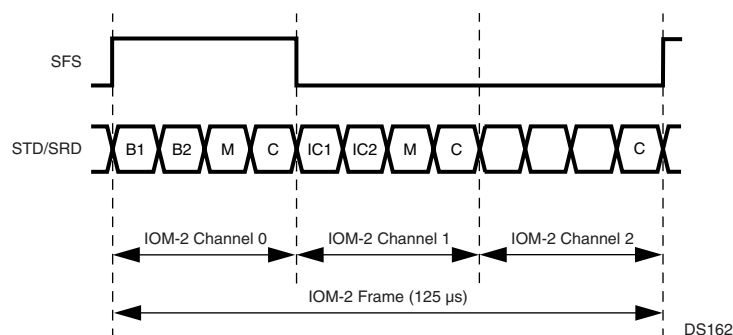
Figure 60. IOM-2 Frame Structure
