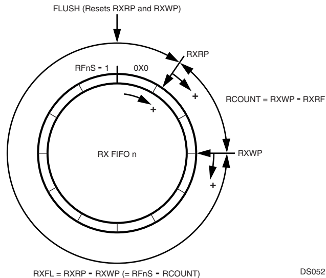
Figure 19. Receive FIFO Operation
