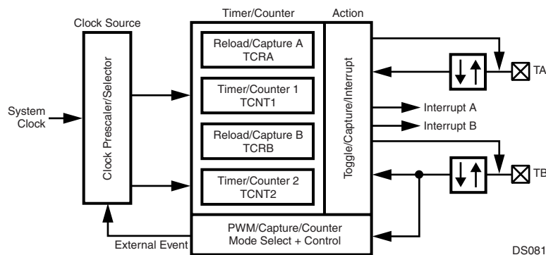
Figure 84. Multi-Function Timer Block Diagram
