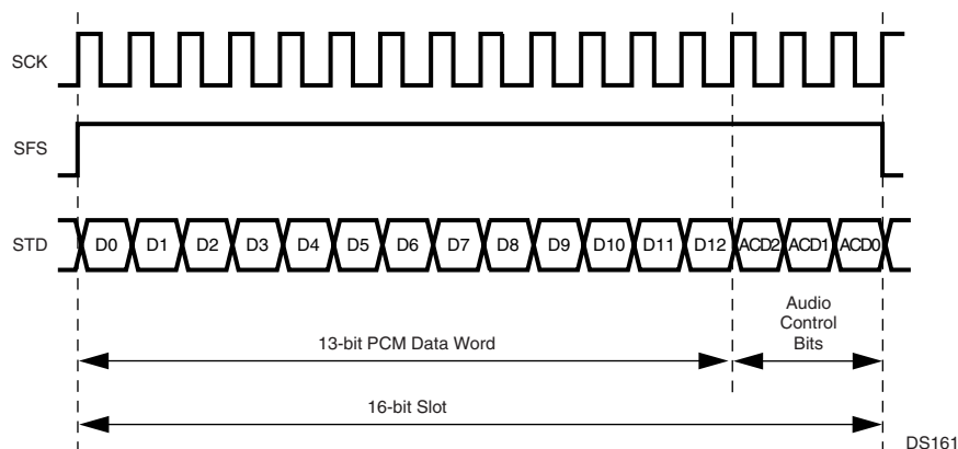
Figure 59. Audio Slot with Audio Control Data
