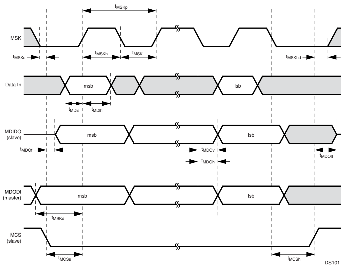
Figure 107. Microwire Transaction Timing, Normal Mode, SCIDL = 0
