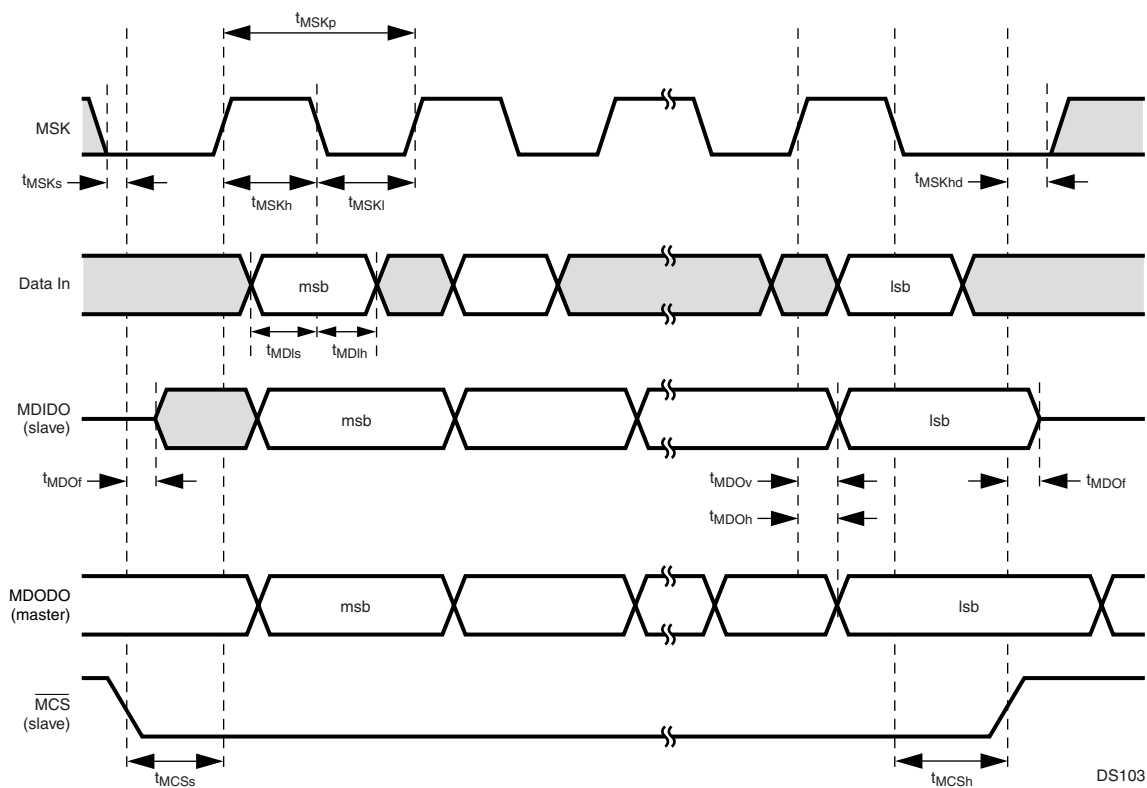
Figure 109. Microwire Transaction Timing, Alternate Mode, SCIDL = 0
