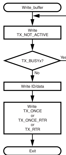
Figure 44. Buffer Write Routine
