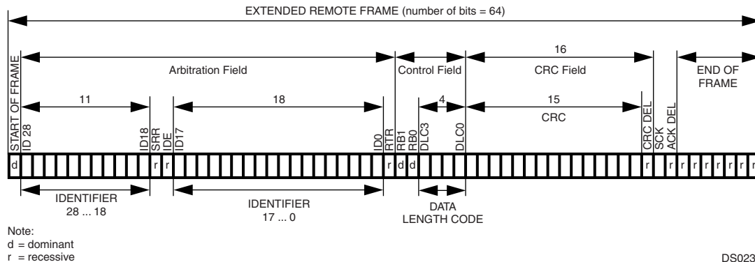
Figure 26. Extended Remote Frame
