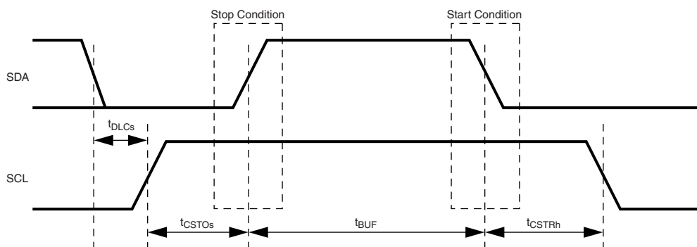
Figure 113. ACB Start and Stop Condition Timing
