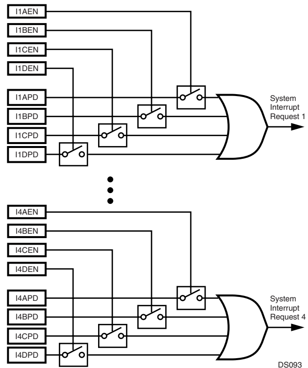
Figure 96. VTU Interrupt Request Structure
