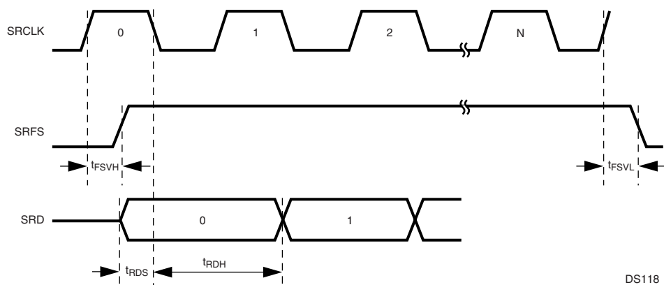
Figure 105. Receive Timing, Long Frame Sync
