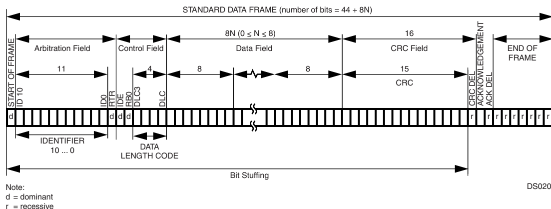
Figure 23. Standard Data Frame
