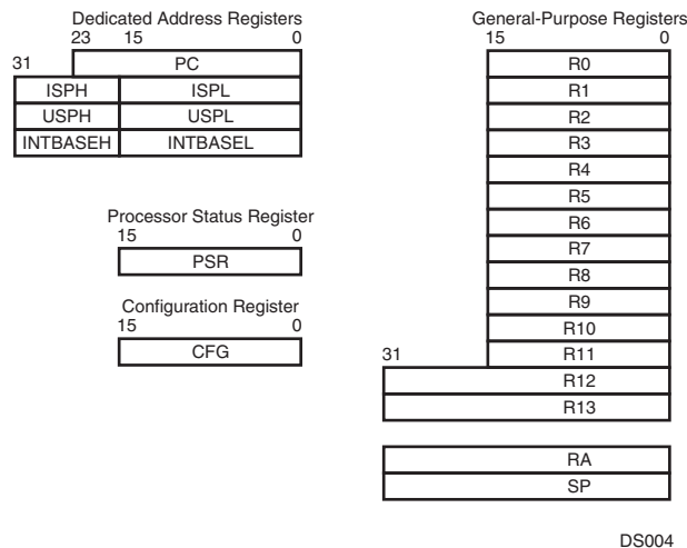
Figure 2. CPU Registers
