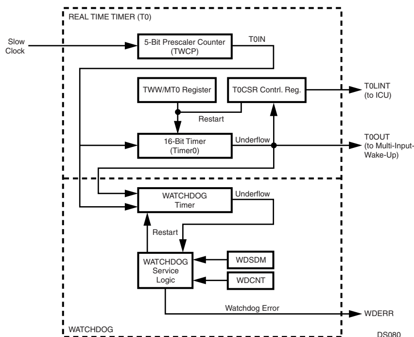
Figure 83. Timing and Watchdog Module Block Diagram
