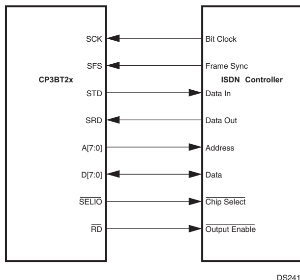
Figure 61. CP3UB26/ISDN Controller Connections
