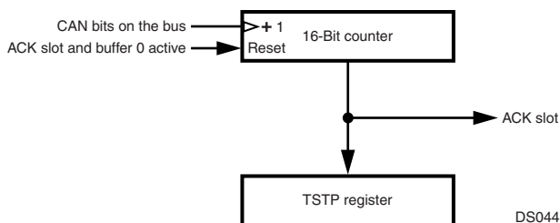
Figure 47. Time Stamp Counter
