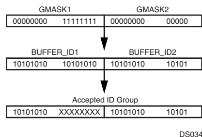
Figure 37. Acceptance of a Group of Identifiers
