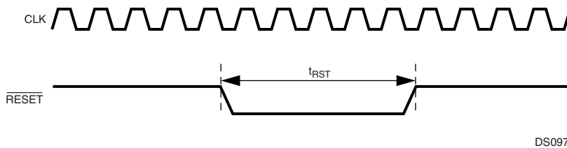
Figure 99. Non-Power-On Reset
