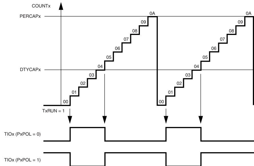
Figure 92. VTU PWM Generation
