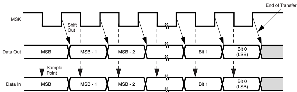
Figure 75. Alternate Mode (SCIDL = 1)
