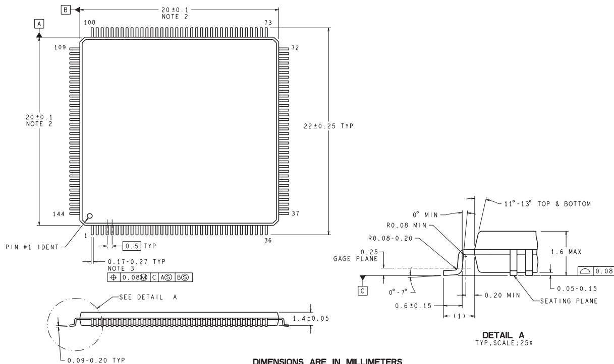
Figure 126. LQFP-144 Package
