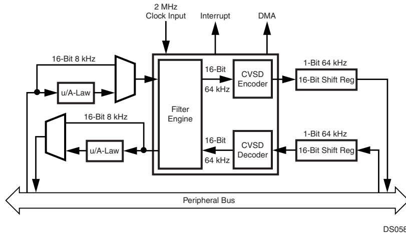
Figure 62. CVSD/PCM Converter Block Diagram
