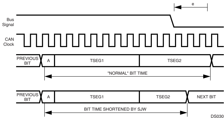
Figure 33. Resynchronization ( e < -SJW )
