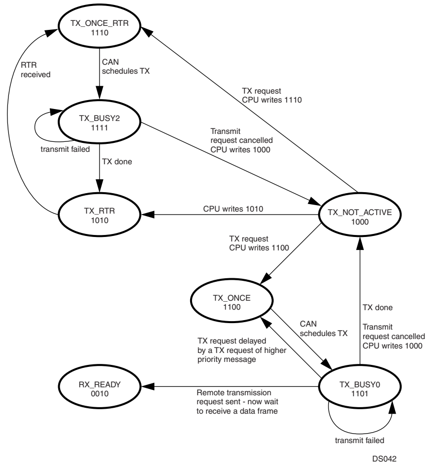
Figure 45. Transmit Buffer States
