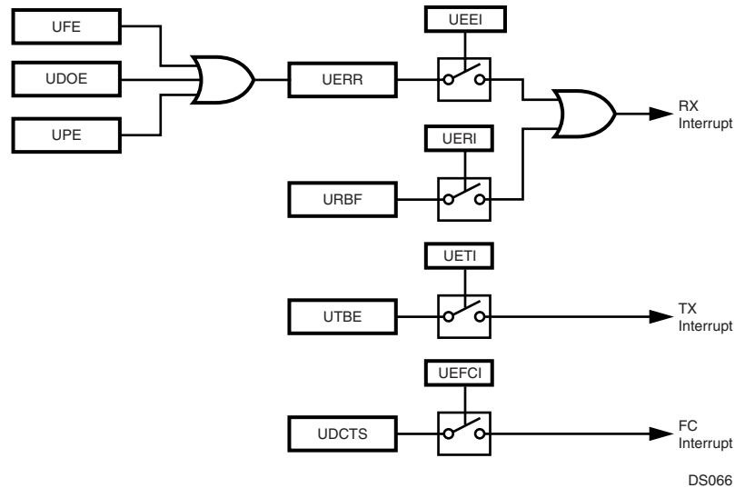
Figure 69. UART Interrupts
