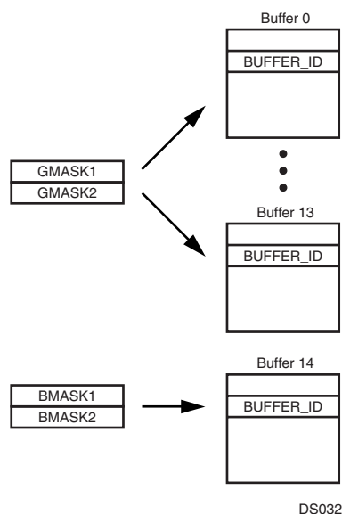
Figure 35. Acceptance Filtering
