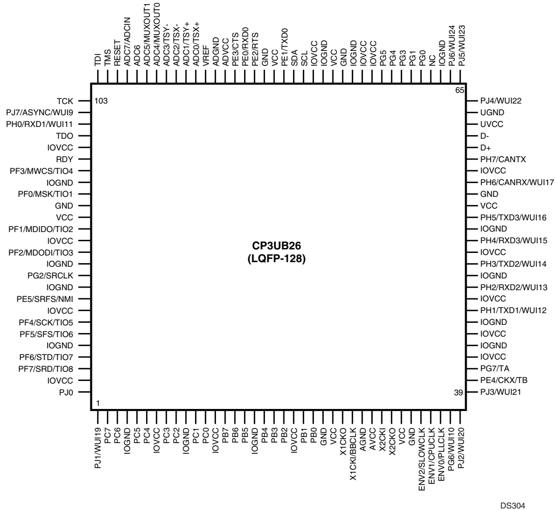
Figure 123. CP3UB26 in the LQFP-128 Package (Top View)
