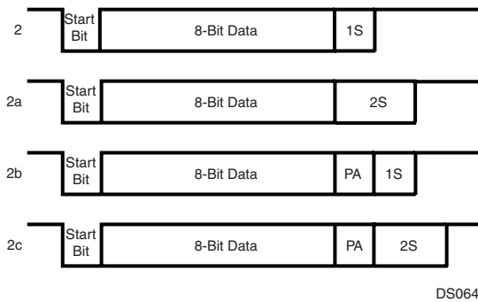
Figure 67. 8-Bit Data Frame Options
