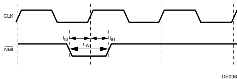
Figure 98. \overline{\text{NMI}} Signal Timing
