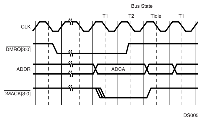
Figure 3. Direct DMA Cycle Followed by a CPU Cycle
