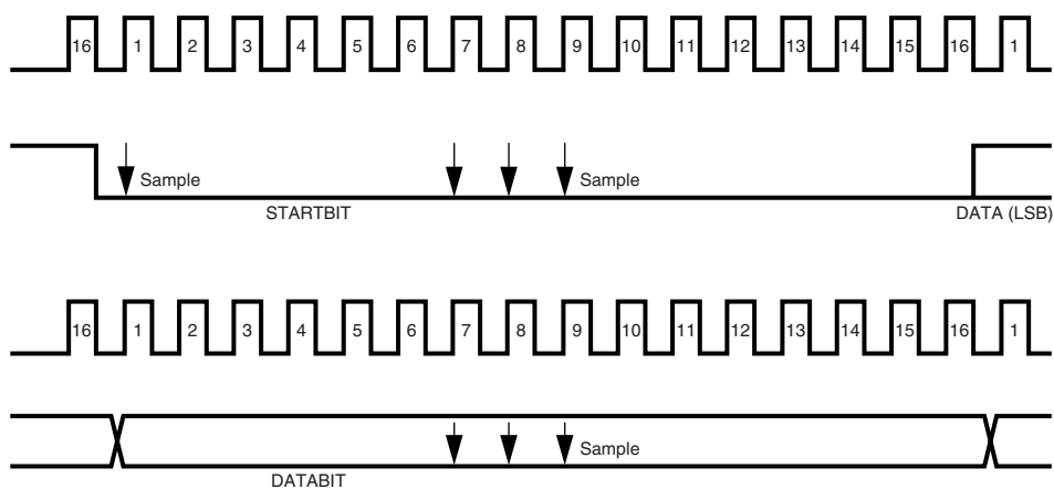
Figure 64. UART Asynchronous Communication
