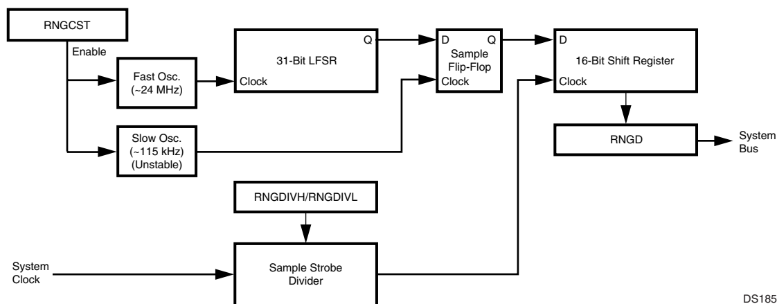
Figure 15. RNG Module Block Diagram
