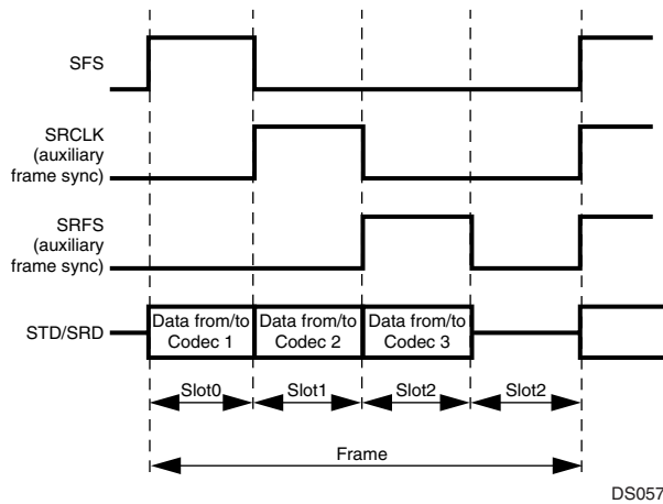
Figure 56. Accessing Three Devices in Network Mode
