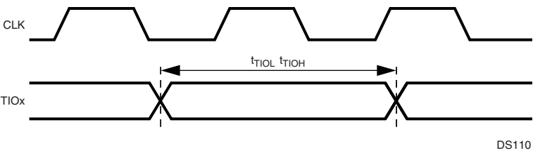
Figure 117. Versatile Timing Unit Input Timing
