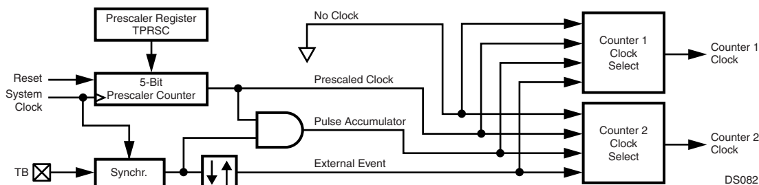
Figure 85. Multi-Function Timer Clock Source
