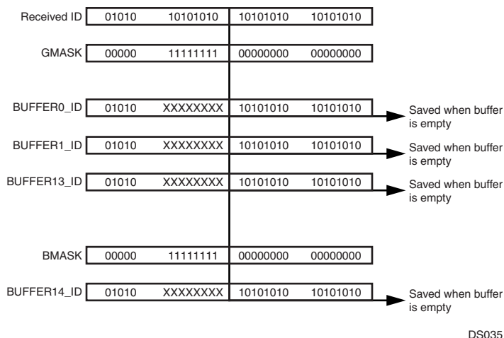
Figure 38. Message Storage with BUFFLOCK Enabled
