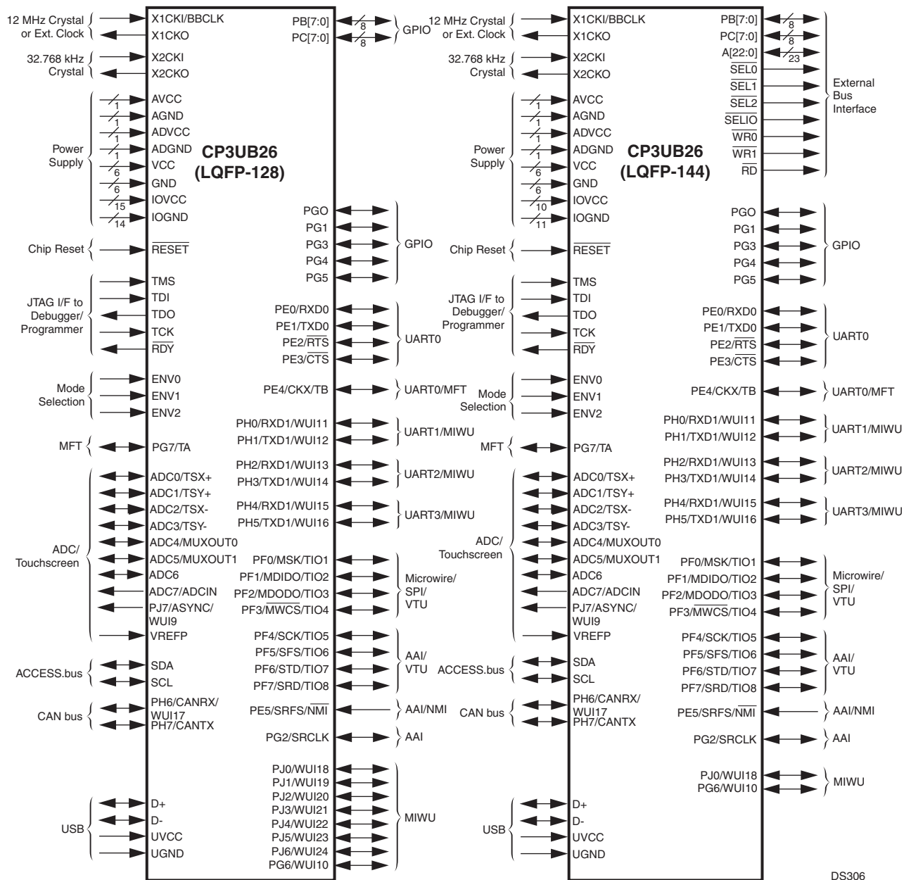
Figure 1. CP3UB26 Device Signals
