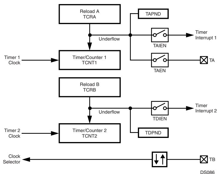
Figure 89. Dual-Independent Timer/Counter Mode
