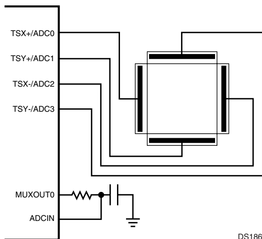
Figure 12. Touchscreen Interface
