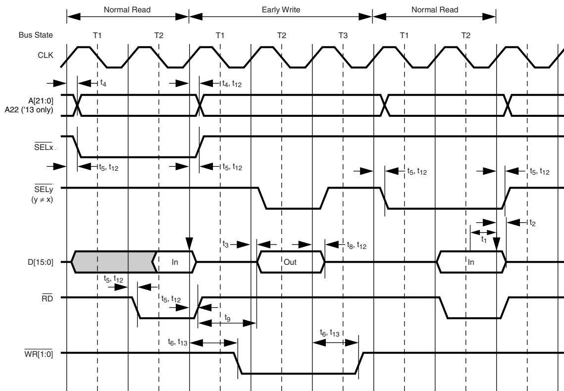
Figure 118. Early Write Between Normal Read Cycles (No Wait States)
