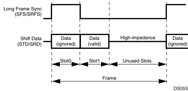
Figure 54. Network Mode Frame
