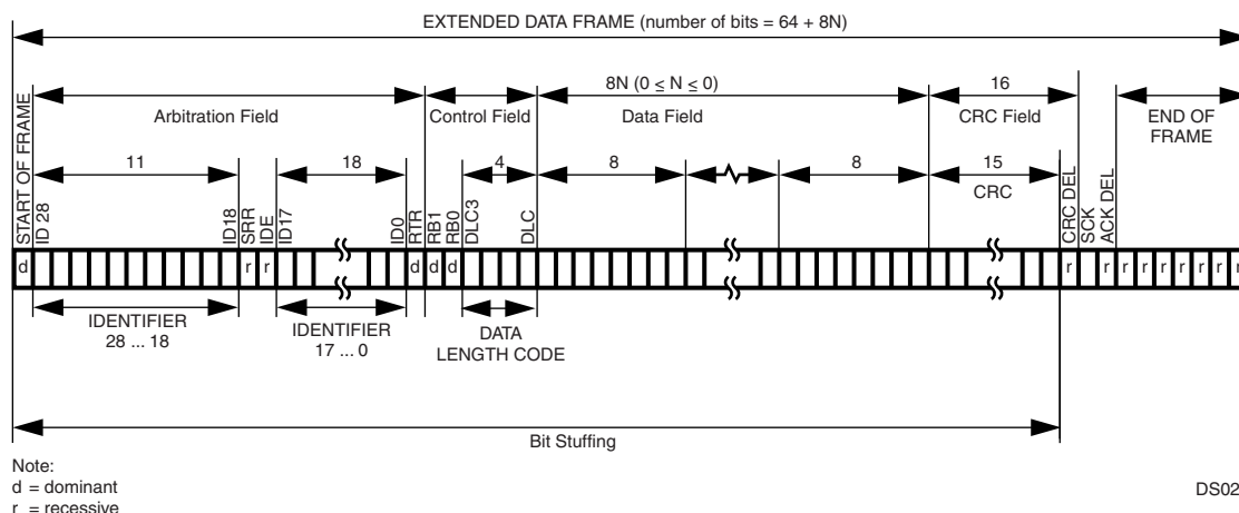
Figure 24. Extended Data Frame
