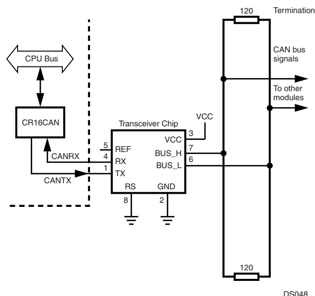
Figure 51. External Transceiver
