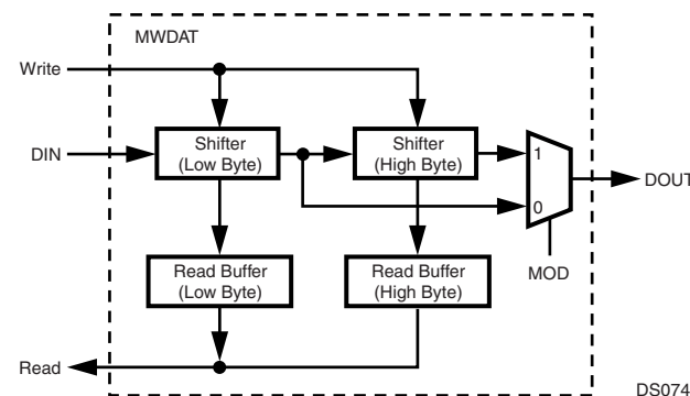
Figure 77. MWDAT Register
