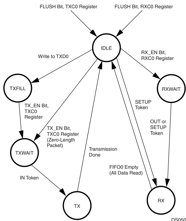
Figure 17. Endpoint 0 Operation
