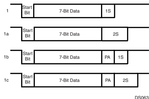
Figure 66. 7-Bit Data Frame Options
