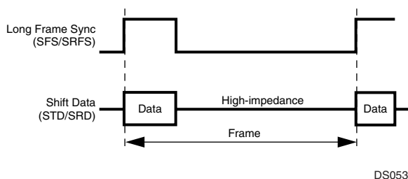
Figure 52. Normal Mode Frame
