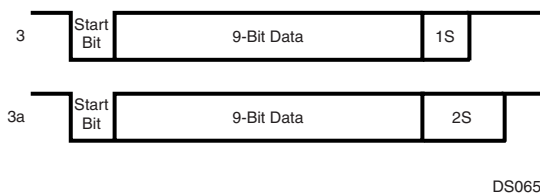
Figure 68. 9-bit Data Frame Options
