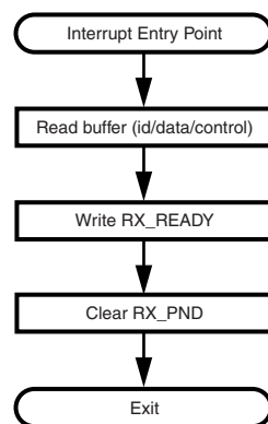
Figure 42. Buffer Read Routine (BUFFLOCK Enabled)
