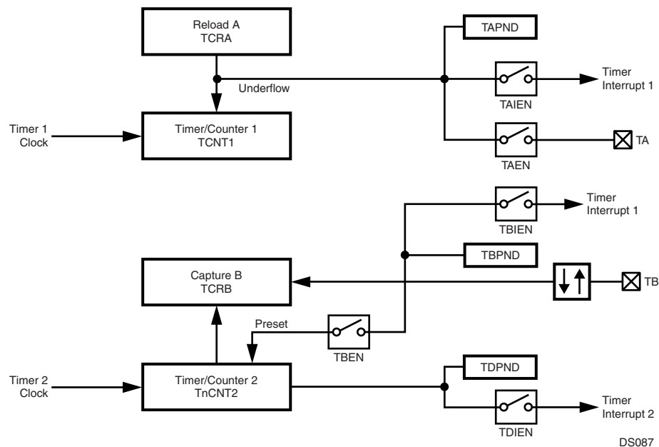
Figure 90. Input Capture Plus Timer Mode
