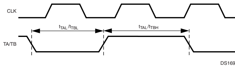
Figure 116. Multi-Function Timer Input Timing
