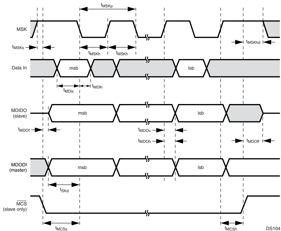
Figure 110. Microwire Transaction Timing, Alternate Mode, SCIDL = 1
