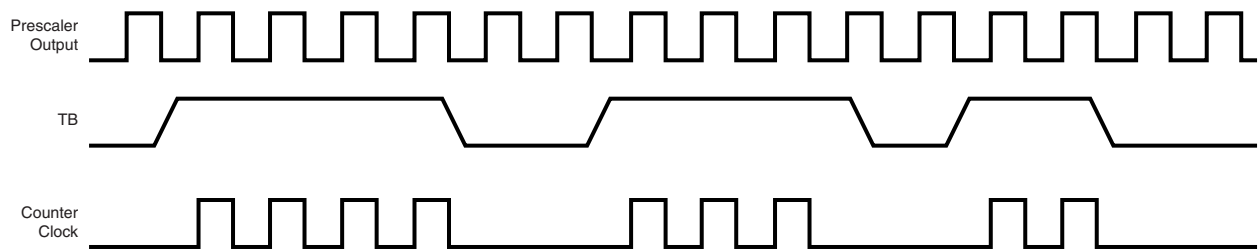
Figure 86. Pulse-Accumulate Mode
