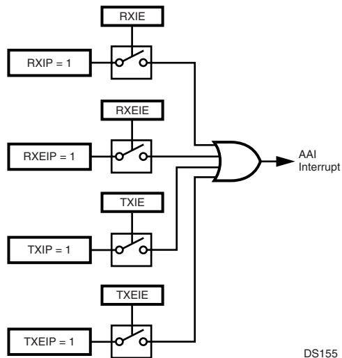
Figure 57. AAI Interrupt Structure
