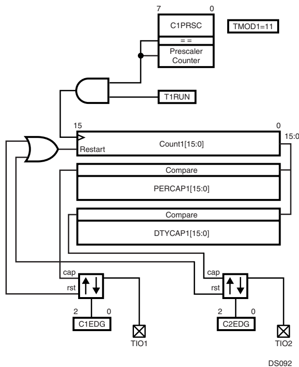
Figure 95. VTU Dual 16-bit Capture Mode
