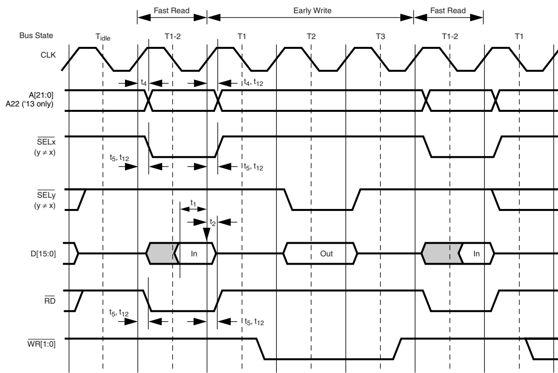
Figure 122. Early Write Between Fast Read Cycles
