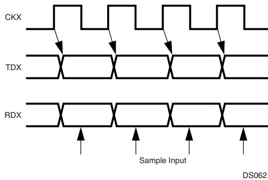
Figure 65. UART Synchronous Communication
