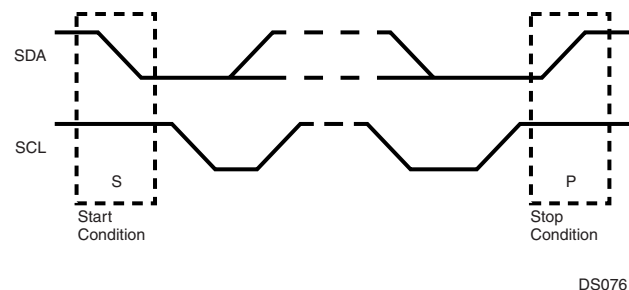
Figure 79. Start and Stop Conditions
