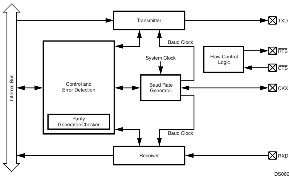
Figure 63. UART Block Diagram
