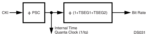
Figure 34. CAN Prescaler
