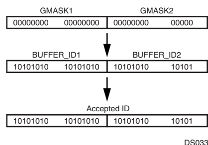
Figure 36. Acceptance of a Single Identifier
