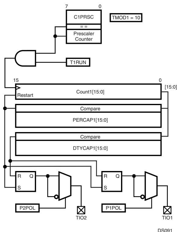
Figure 94. VTU 16-bit PWM Mode
