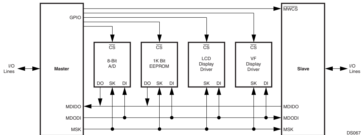
Figure 70. Microwire Interface
