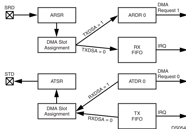
Figure 53. IRQ/DMA Support in Normal Mode
