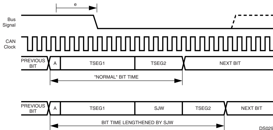
Figure 32. Resynchronization ( e > SJW )
