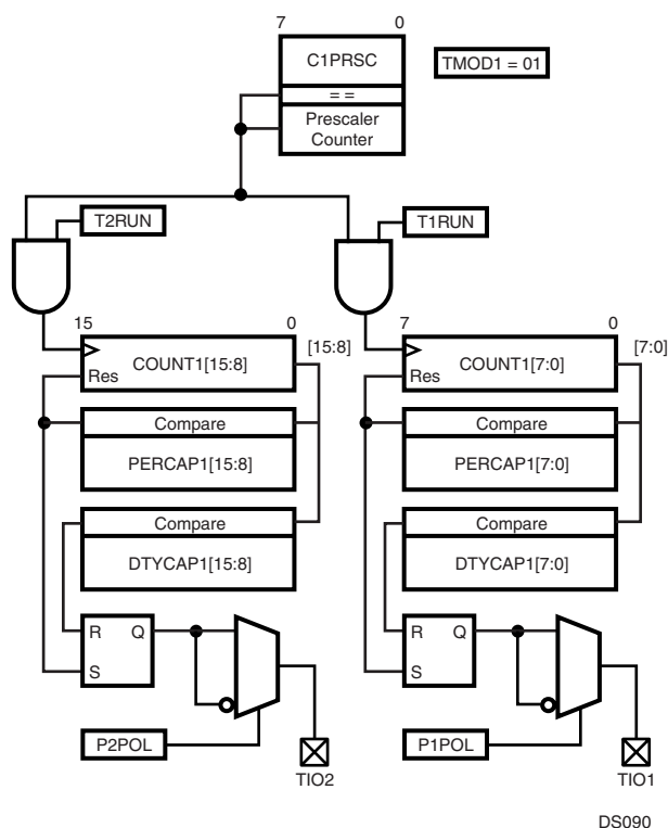
Figure 93. VTU Dual 8-Bit PWM Mode
