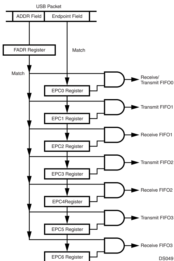
Figure 16. USB Function Address/Endpoint Decoding
