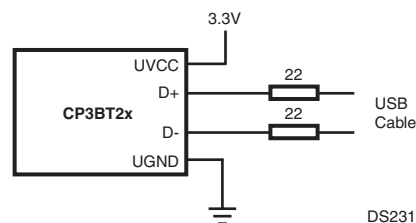
Figure 20. USB Transceiver Interface
