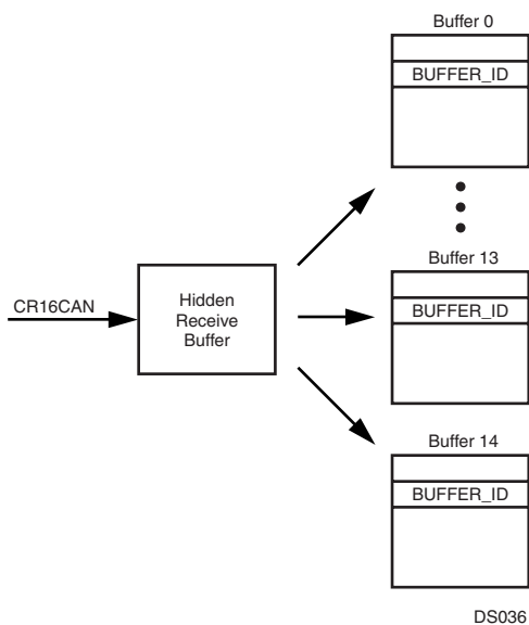
Figure 39. Receive Buffer
