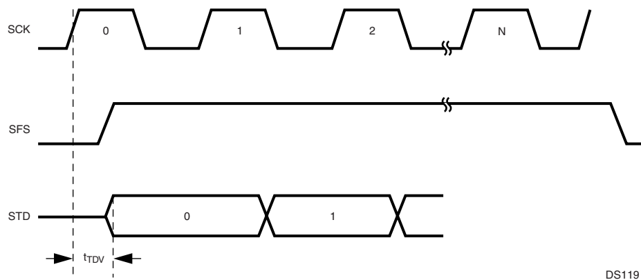
Figure 106. Transmit Timing, Long Frame Sync
