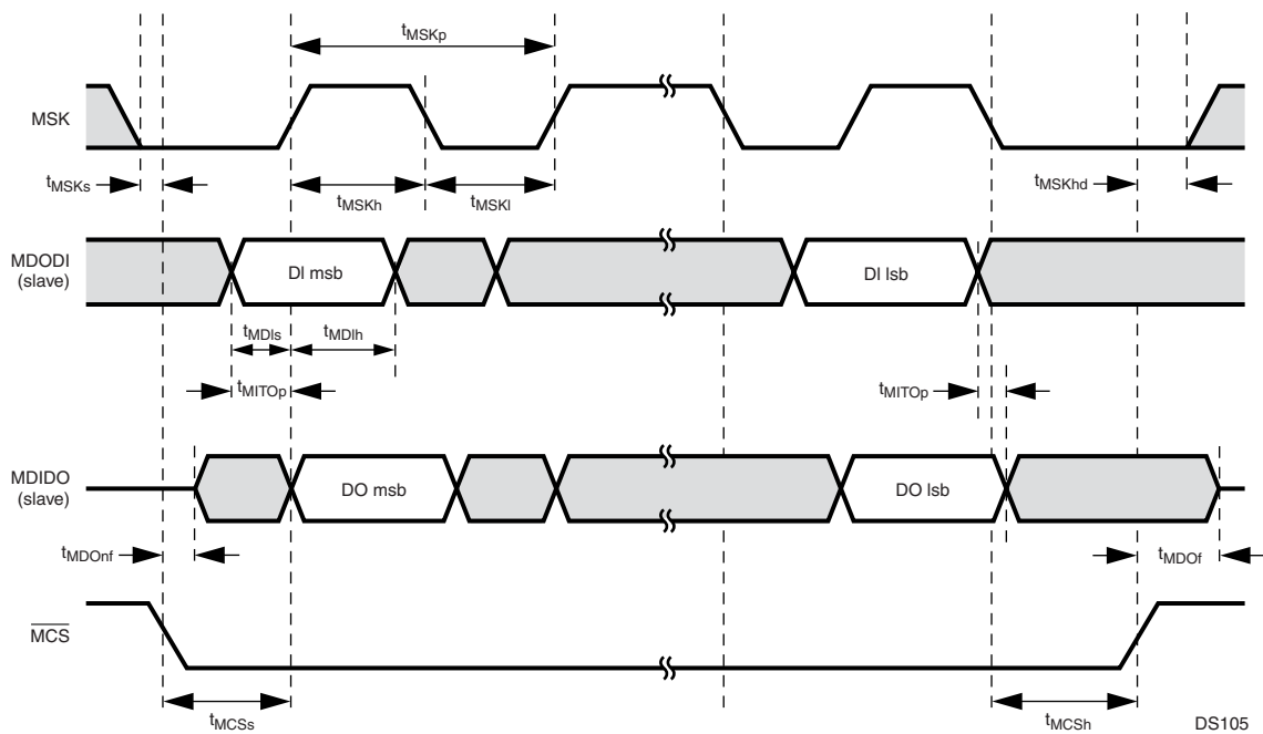
Figure 111. Microwire Transaction Timing, Data Echoed to Output, Normal Mode, SCIDL = 0, ECHO = 1, Slave Mode
