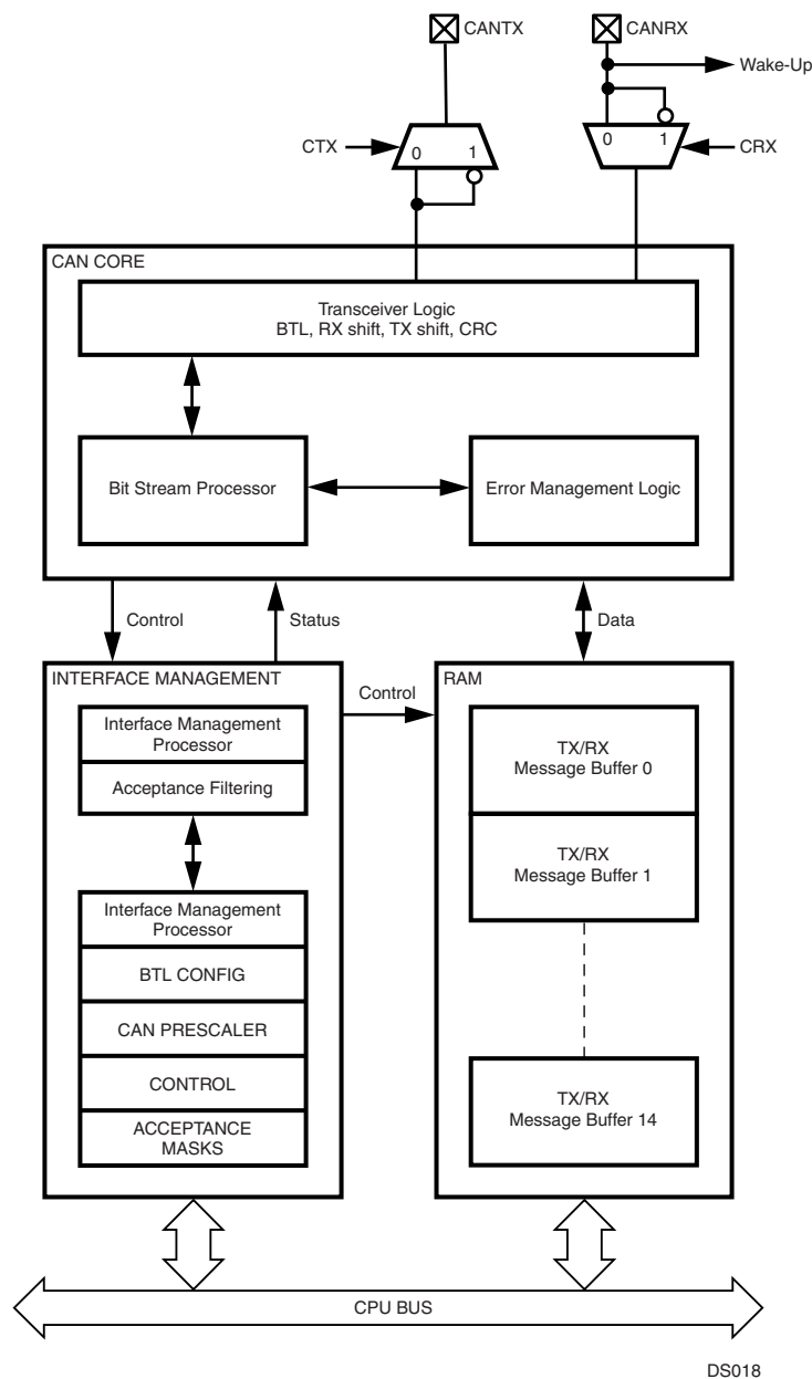
Figure 21. CAN Block Diagram
