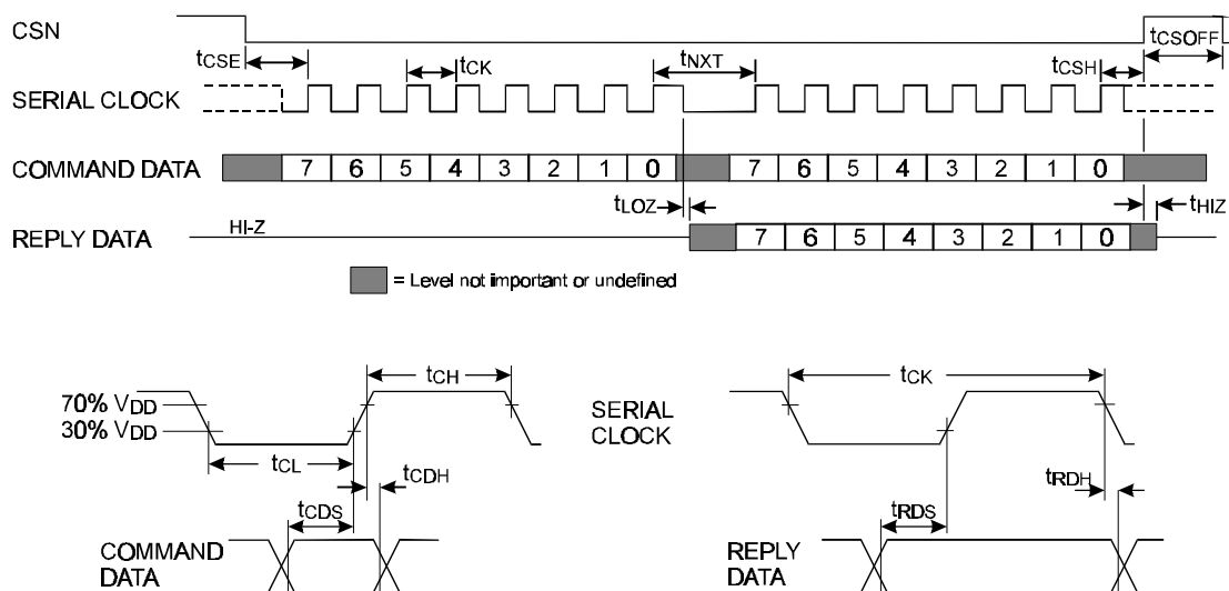
Figure 10 'C-BUS' Timing
