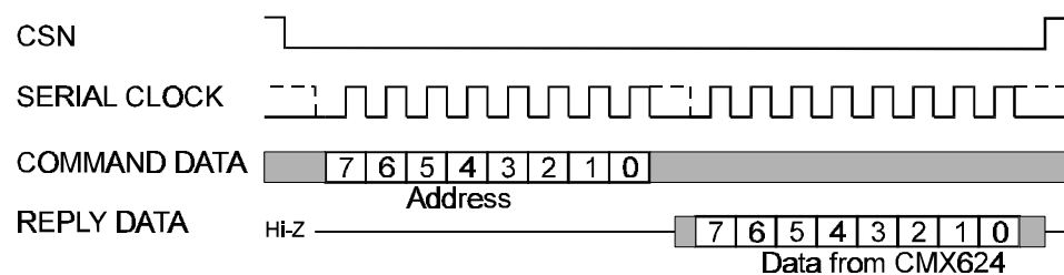
Figure 7 'C-BUS' Transactions
