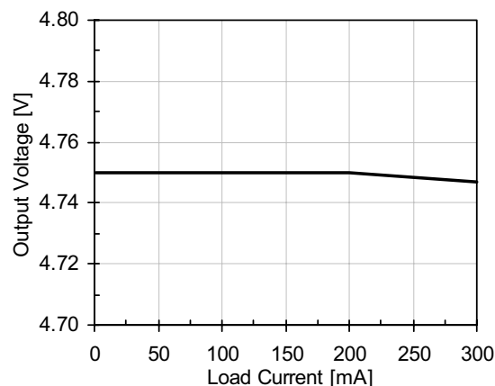
Load Regulation
