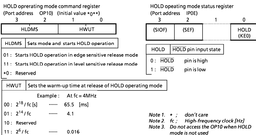
Figure 2-21. HOLD Operating Mode Command Register/Status Register
