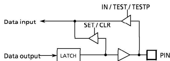
Figure 3-5. Ports R4, R5, R6
