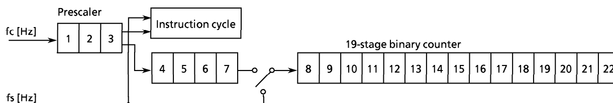
Figure 2-16. Configuration of Timing Generator
