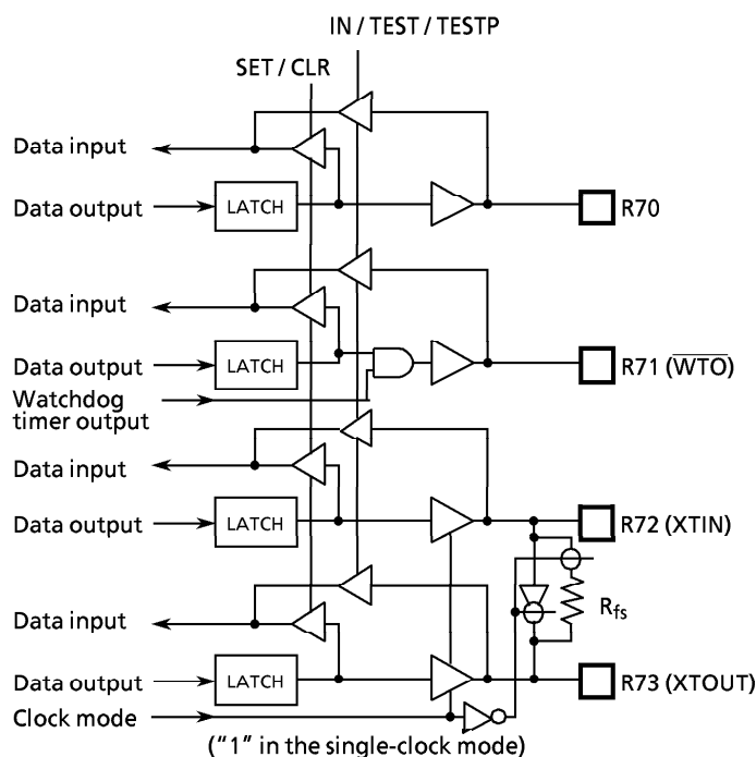
Figure 3-6. Port R7
