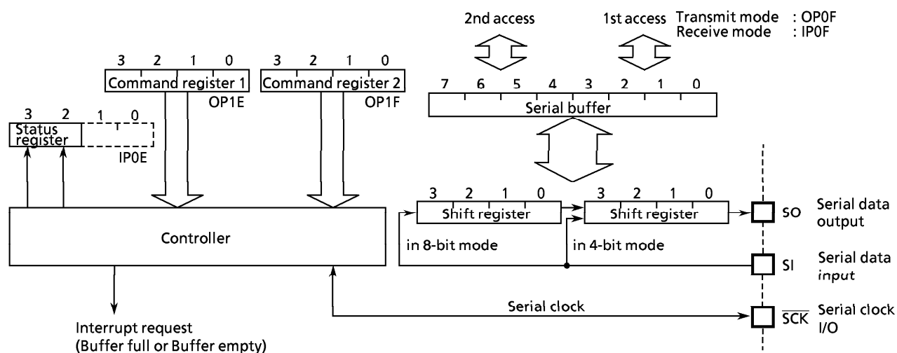
Figure 3-19. Configuration of Serial Interface
