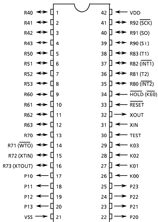
(1) SDIP42-P-600-1.78
