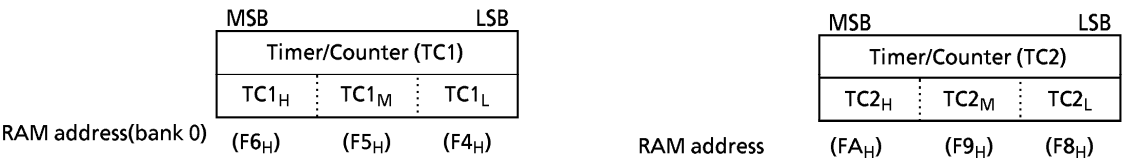
Figure 3-11. Count Registers of the Timer/Counters (TC1, TC2)
