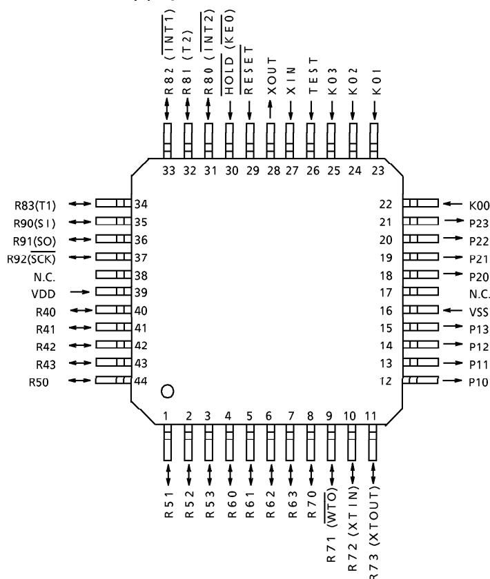
(2) QFP44-P-1414-0.80D
