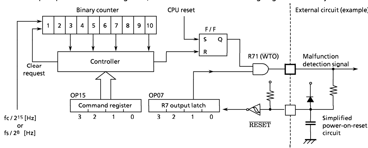
Figure 3-17. Configuration of Watchdog Timer
