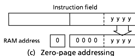
Figure 2-5. Addressing mode
