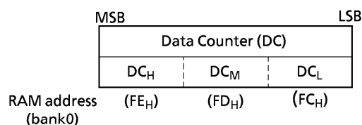
Figure 2-8. Data Counter
