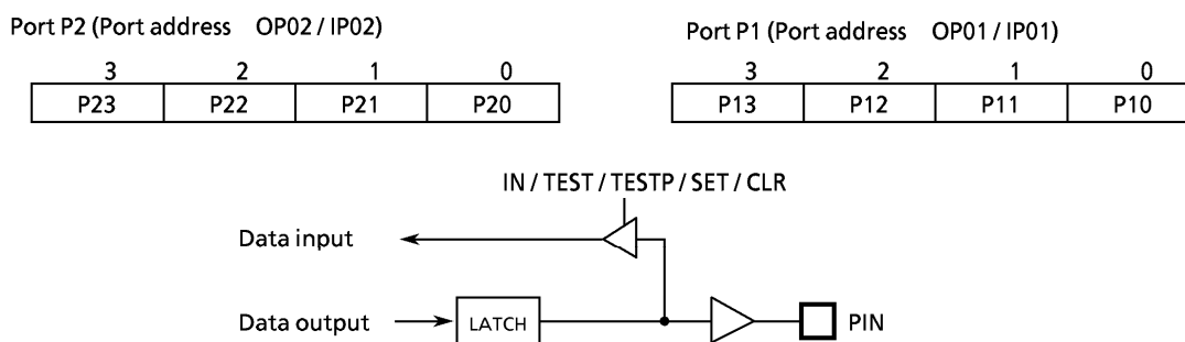
Figure 3-4. Ports P1, P2
