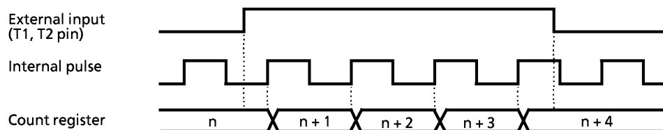
Figure 3-16. Pulse Width Measurement Mode Timing Chart
