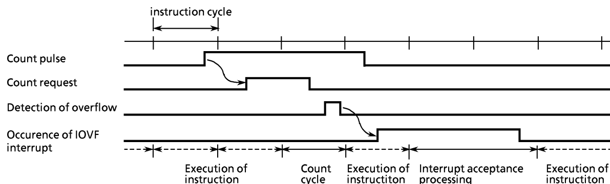
Figure 3-13. Timer/Counter Overflow Interrupt Timing
