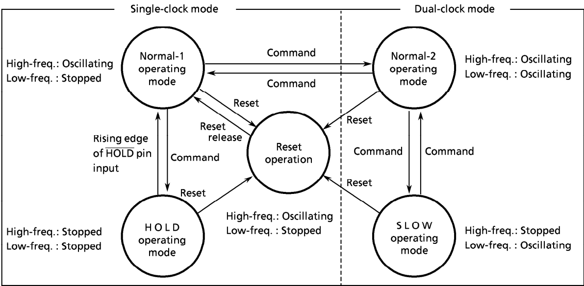
Figure 2-17. Operating Mode Transition Diagram
