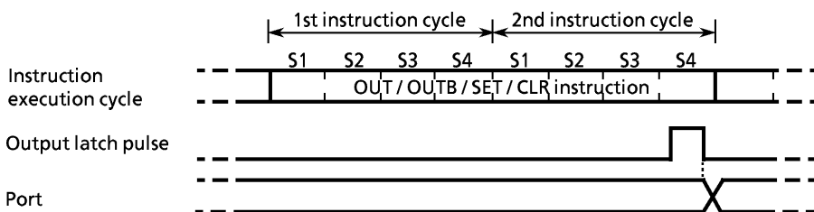
Figure 3-2. Output Timing
