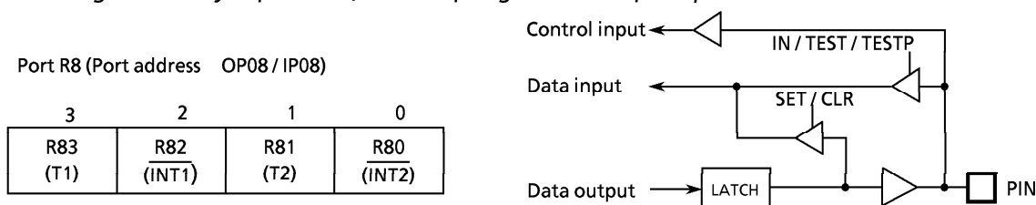
Figure 3-7. Port R8
