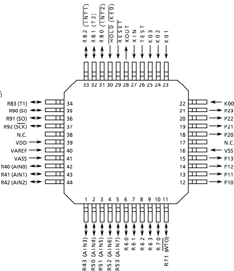
(2) QFP44-P-1414-0.80D
