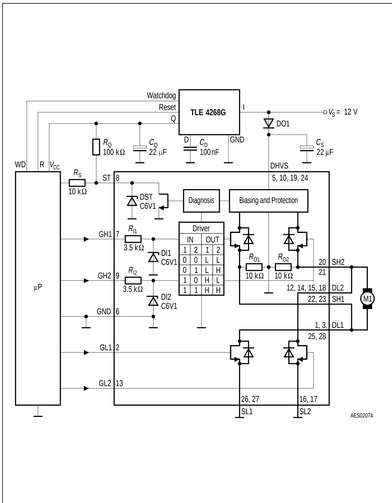
Figure 4 Application Circuit
