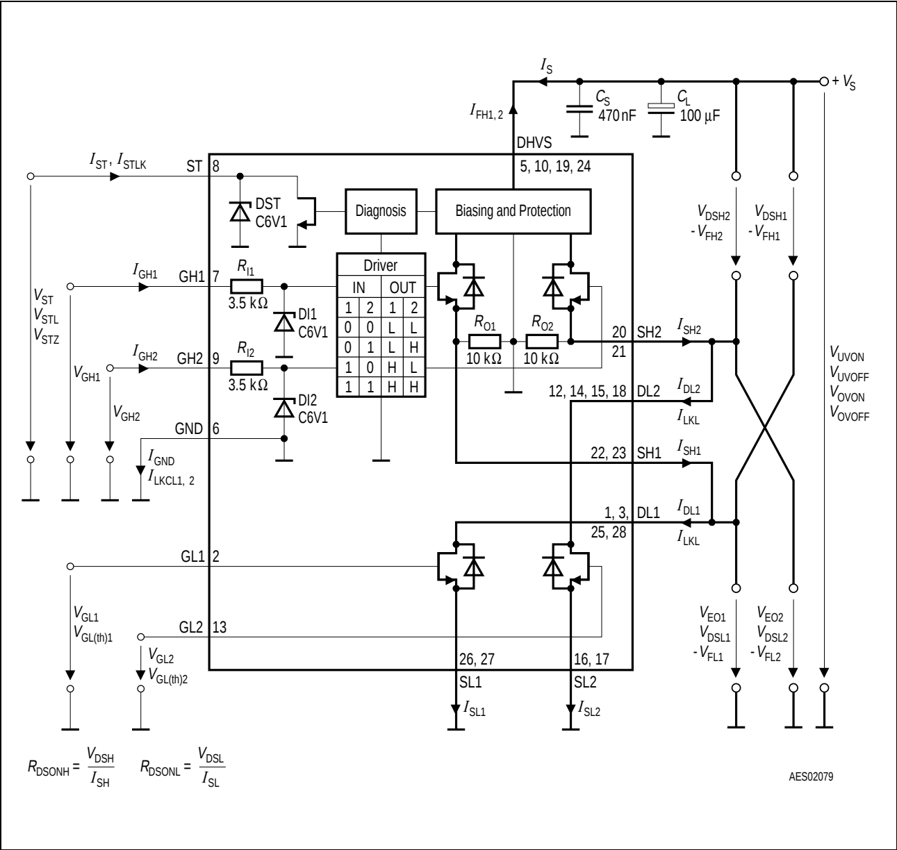
Figure 3 Test Circuit
