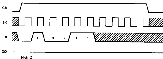
Fig. 3 Write enable cycle timing
