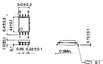
SSOP-B8
