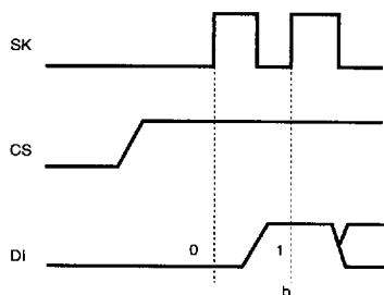
Fig. 9 Normal operation timing
