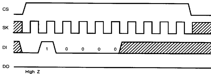
Fig. 6 Write disable cycle timing (WDS)
