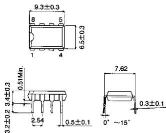
DIP8
