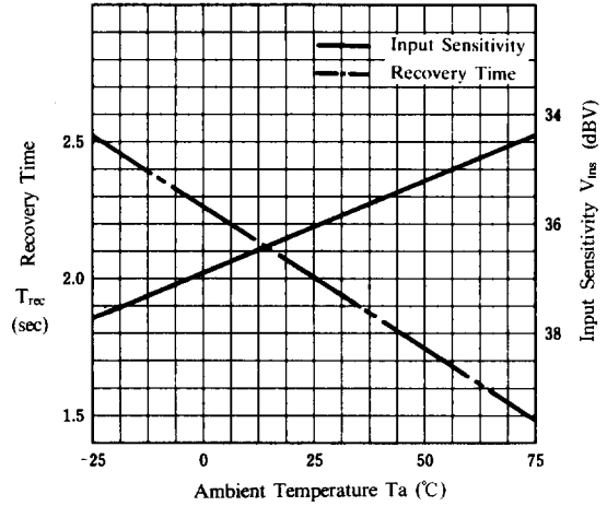
Input Sensitivity Recovery Time vs. Ambient Temperature
