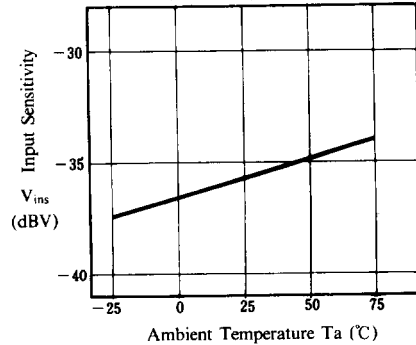
Input Sensitivity vs. Ambient Temperature
