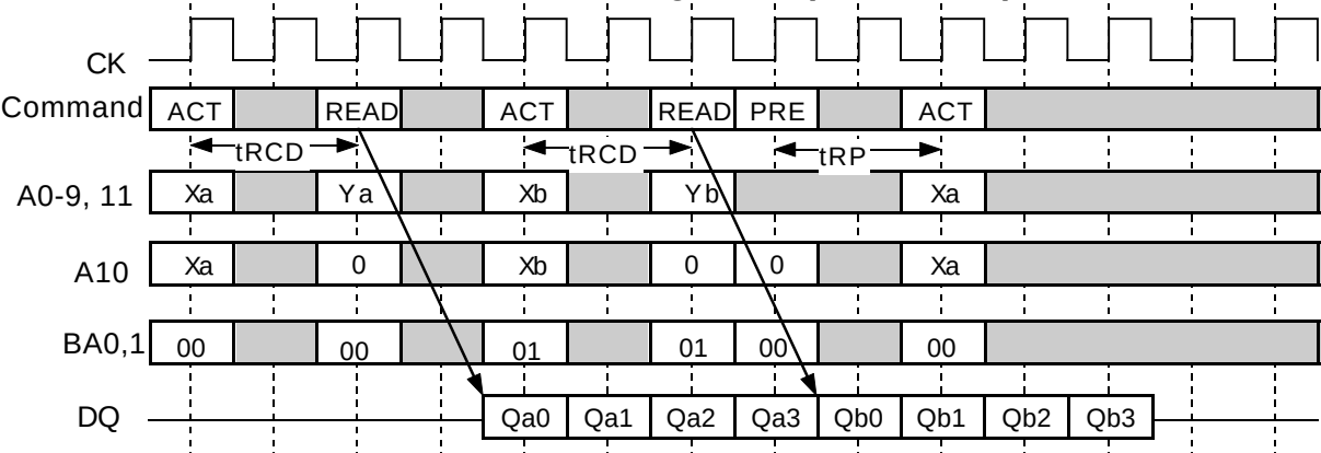
Multi Bank Interleaving READ (BL=4, CL=2)
