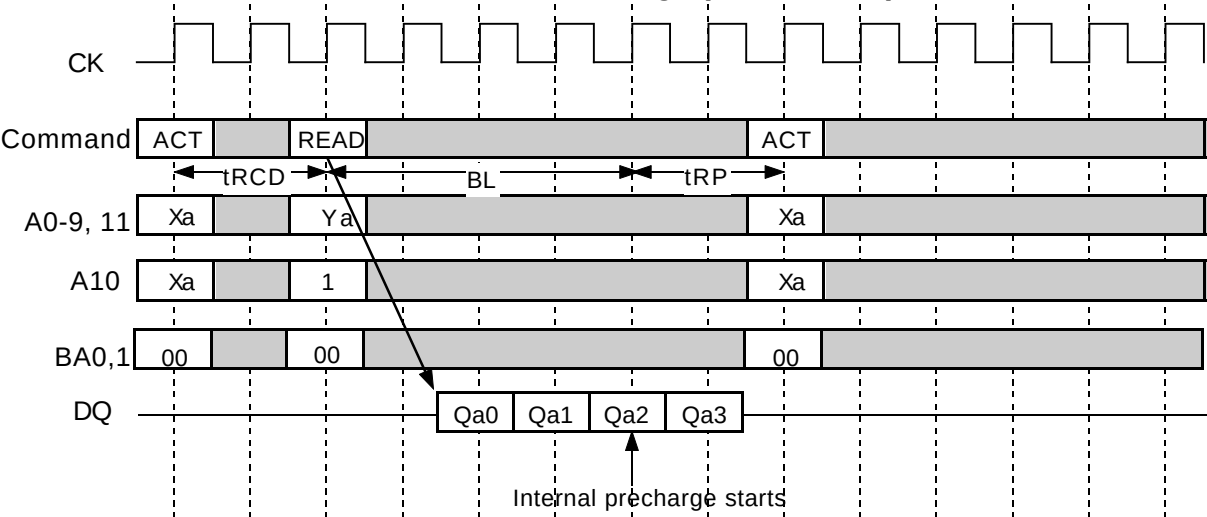
READ with Auto-Precharge (BL=4, CL=2)
