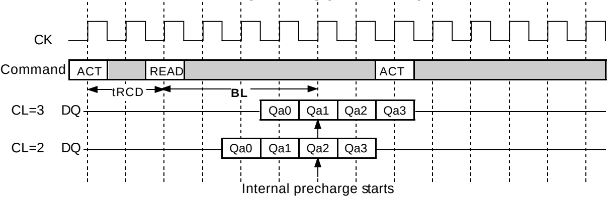
Auto-Precharge Timing (READ BL=4)
