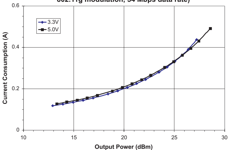
Figure 4: Typical Current vs. Output Power ( T_A = +25\text{ }^{\circ}\text{C} , V_{REF1} = V_{REF2} = +2.85\text{ V} ) 802.11g modulation, 54 Mbps data rate)
