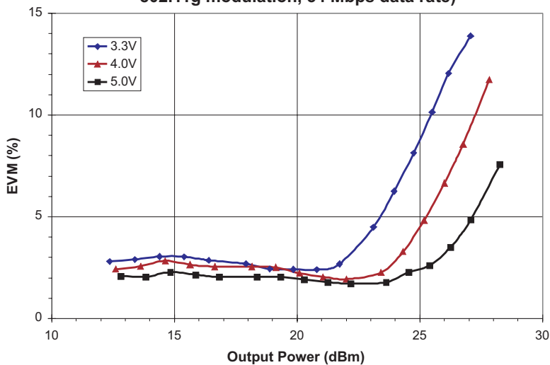
Figure 3: Typical EVM (1) vs. Output Power ( T_A = +25\text{ }^{\circ}\text{C} , V_{REF1} = V_{REF2} = +2.85\text{ V} ) 802.11g modulation, 54 Mbps data rate)
