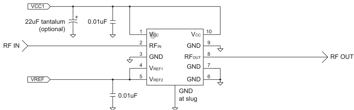
Figure 5: Application Circuit
