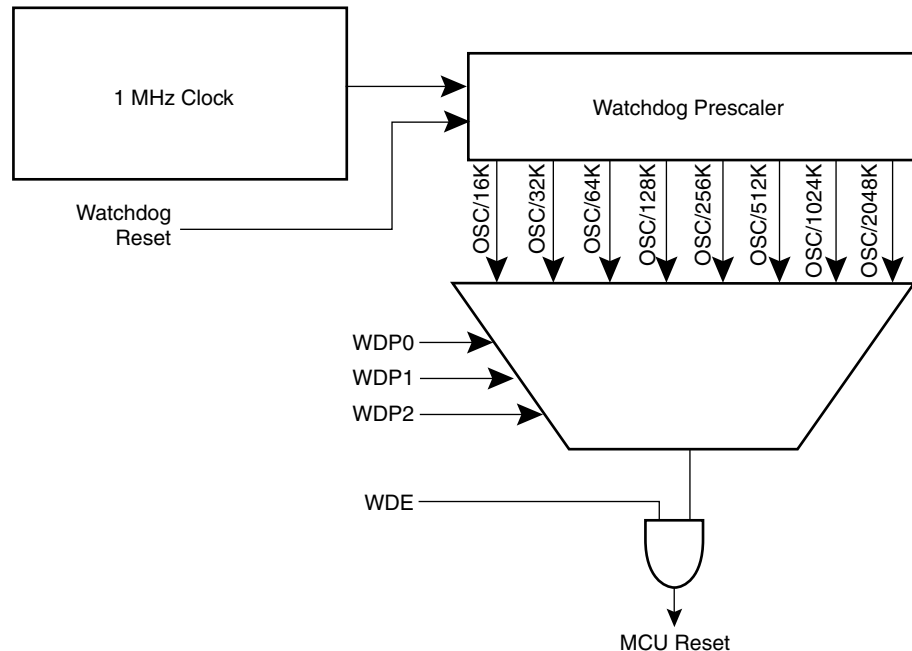
Figure 16. Watchdog Timer
