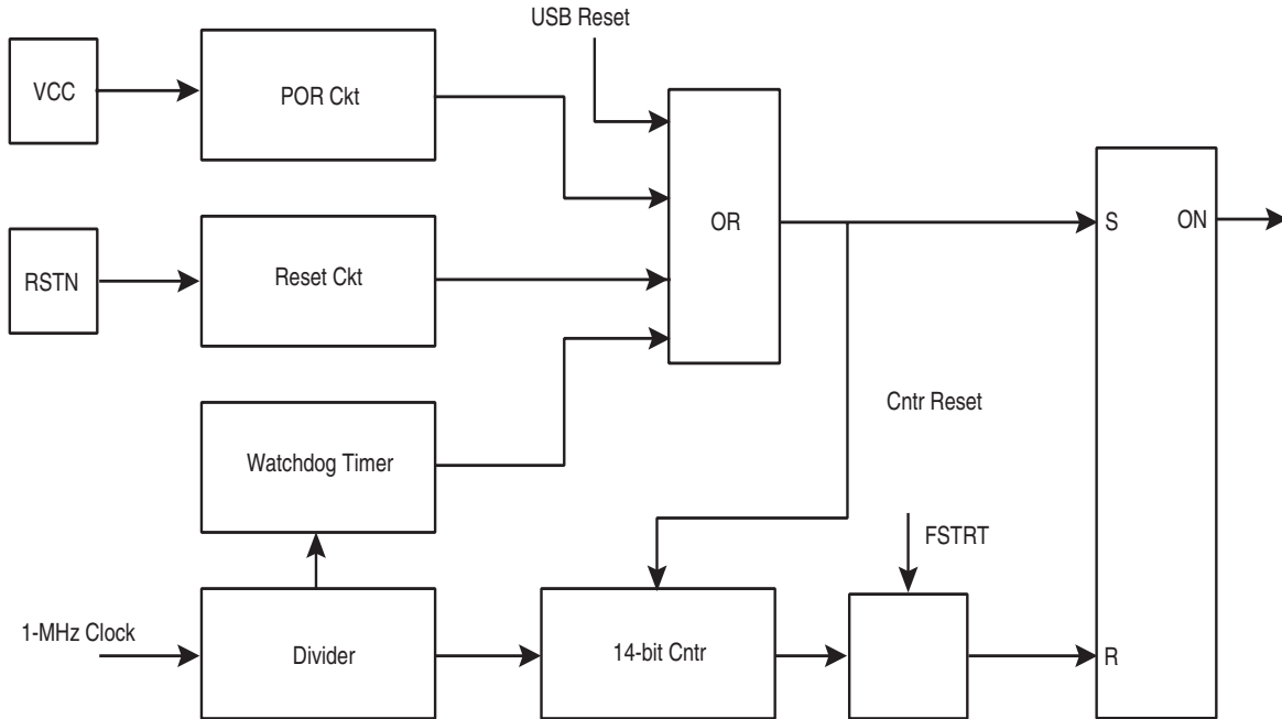
Figure 8. Reset Logic
