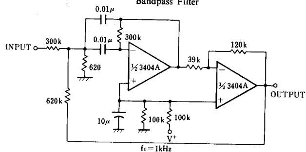
Bandpass Filter
