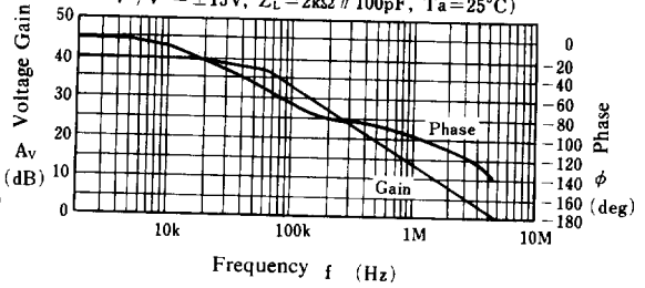
NJM072/082
