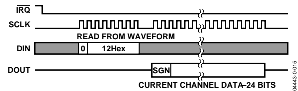
Figure 39. Current Channel Waveform Sampling
