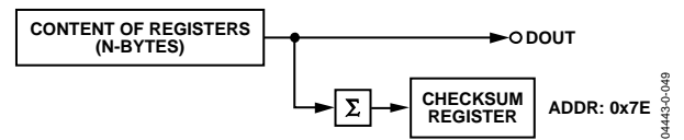
Figure 82. Checksum Register for Serial Interface Read
