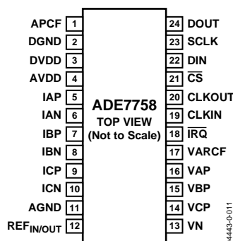
Figure 35. Pin Configuration
