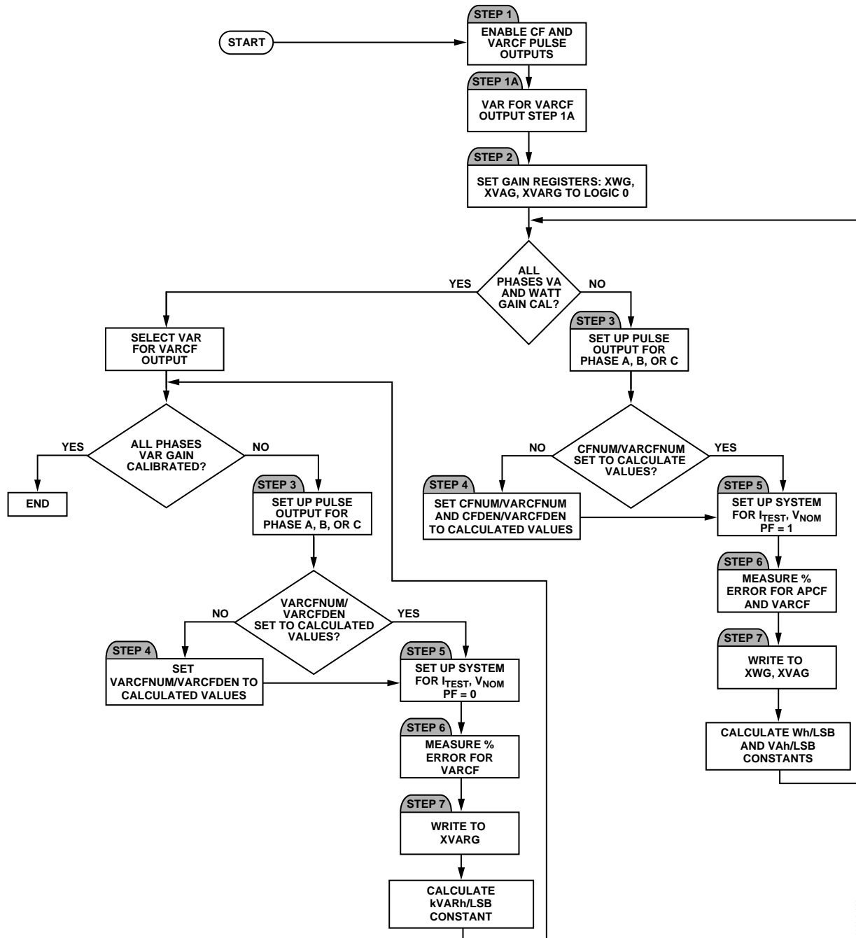
Figure 74. Gain Calibration Using Pulse Output
