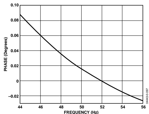
Figure 53. Gain Response of HPF and Phase Compensation (Deviation of Gain as Percent of Gain at 54 Hz)
