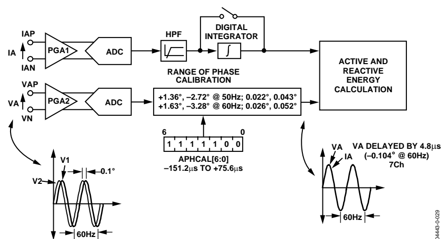
Figure 54. Phase Calibration on Voltage Channels
