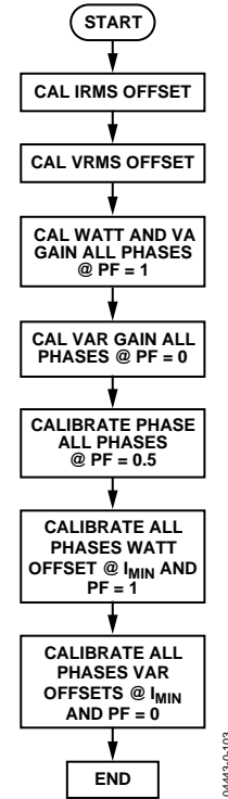
Figure 77. Calibration Using Line Accumulation
