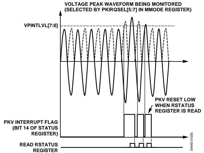
Figure 57. ADE7758 Overcurrent Detection
