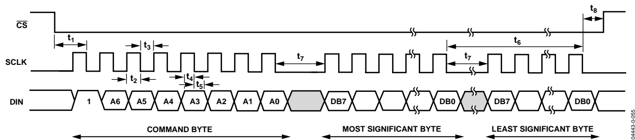
Figure 88. Serial Interface Write Timing Diagram
