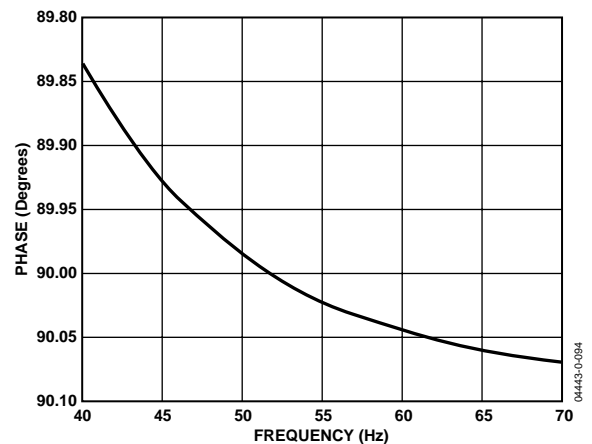
Figure 44. Combined Phase Response of the Digital Integrator and Phase Compensator (40 Hz to 70 Hz)
