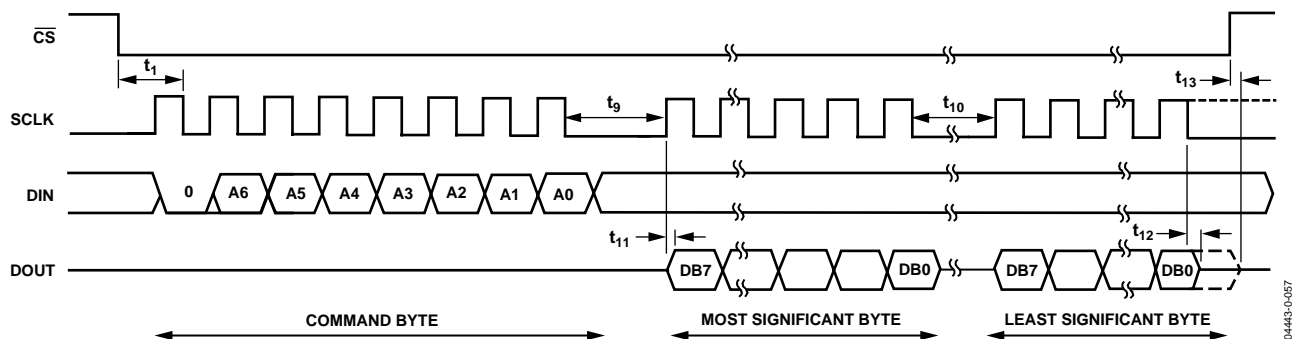
Figure 90. Serial Interface Read Timing Diagram
