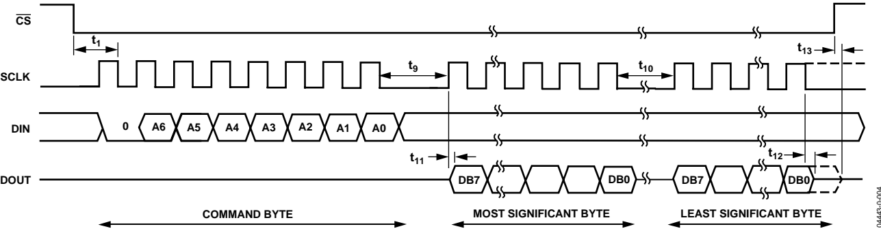
Figure 4. Serial Read Timing
