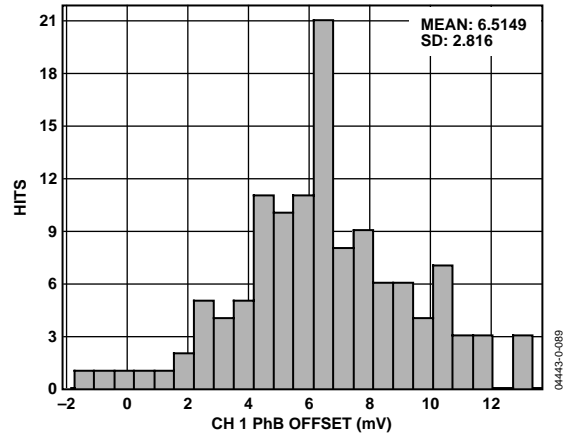
Figure 31. Phase B Channel 1 Offset Distribution
