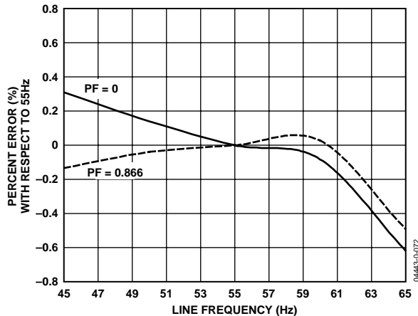
Figure 16. Reactive Energy Error as a Percentage of Reading (Gain = +1) over Frequency with Internal Reference and Integrator Off
