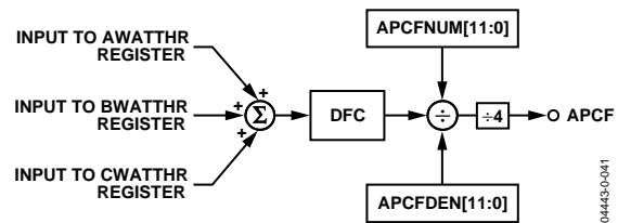
Figure 65. ADE7758 Active Power Frequency Output
