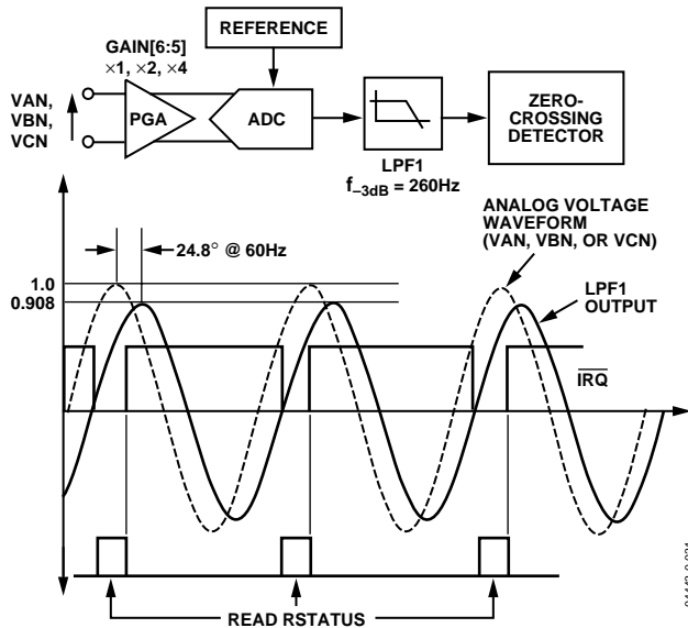
Figure 49. Zero-Crossing Detection on Voltage Channels
