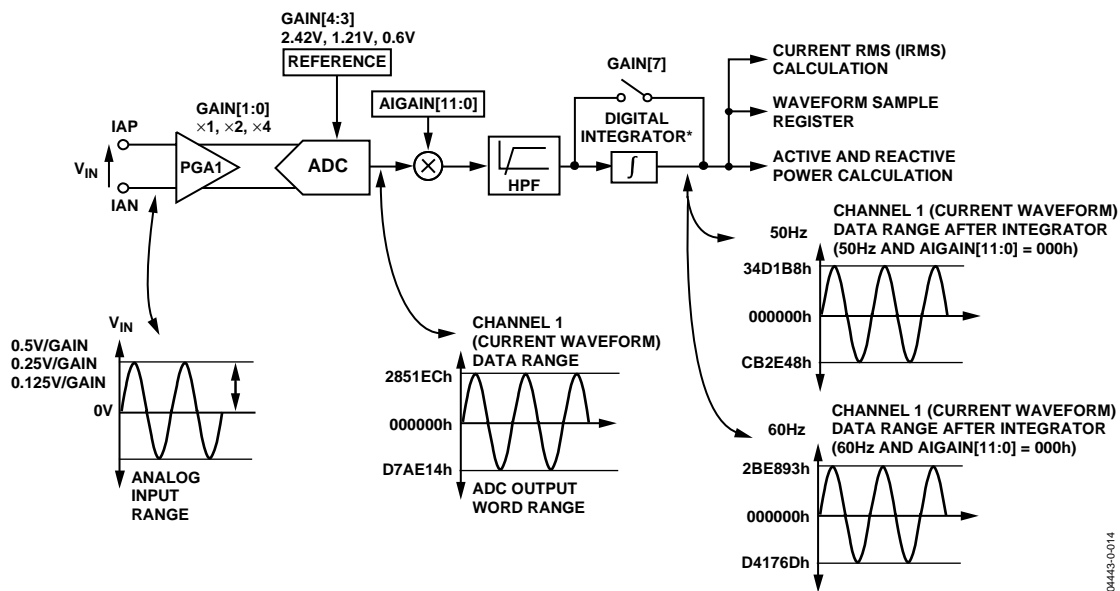
Figure 38. Current Channel Signal Path
