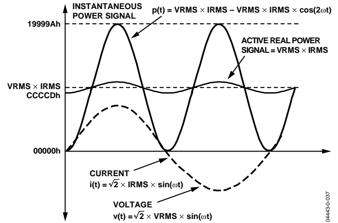
Figure 61. Active Power Calculation
