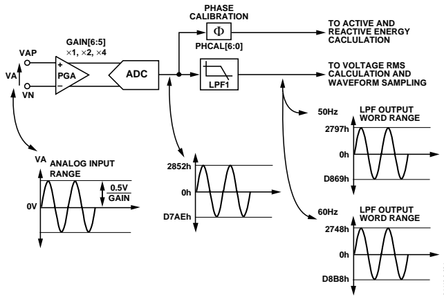
Figure 47. ADC and Signal Processing in Voltage Channel
