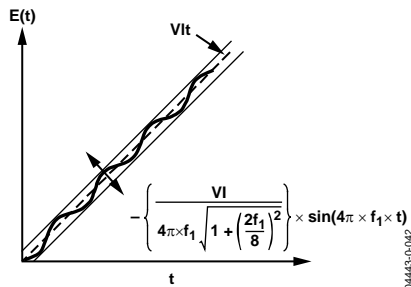
Figure 66. Output Frequency Ripple
