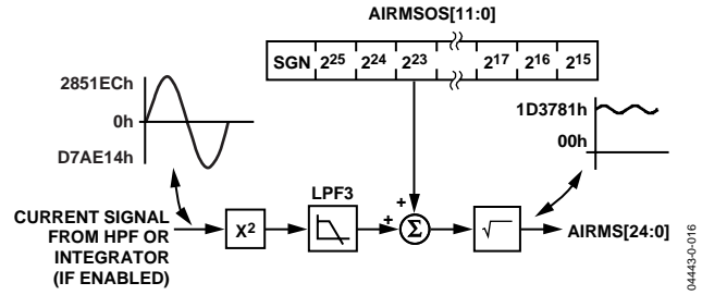
Figure 59. Current RMS Signal Processing
