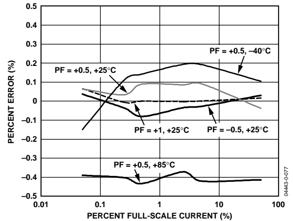
Figure 20. Active Energy Error as a Percentage of Reading (Gain = +4) over Temperature with Internal Reference and Integrator On
