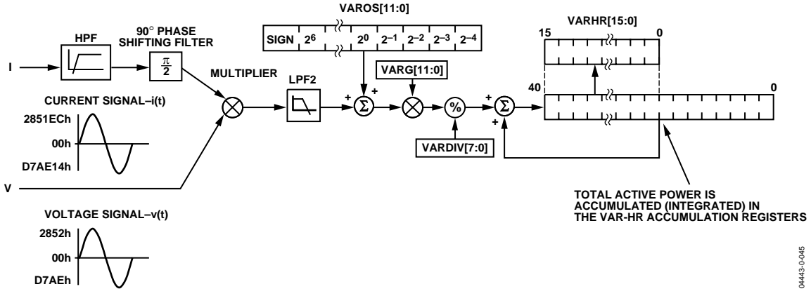
Figure 69. ADE7758 Reactive Energy Accumulation
