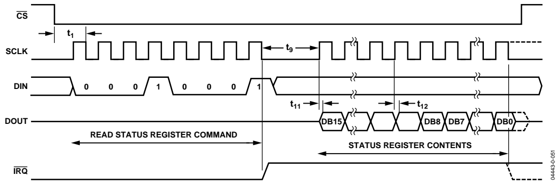
Figure 84. ADE7758 Interrupt Timing
