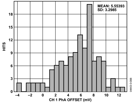
Figure 30. Phase A Channel 1 Offset Distribution
