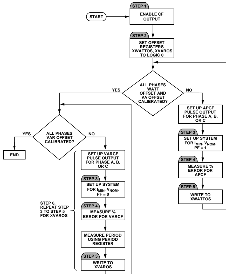
Figure 76. Offset Calibration Using Pulse Output
