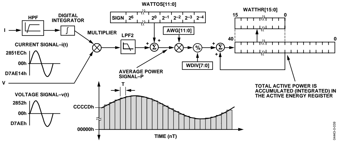
Figure 63. ADE7758 Active Energy Accumulation
