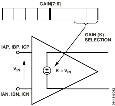
Figure 36. PGA in Current Channel
