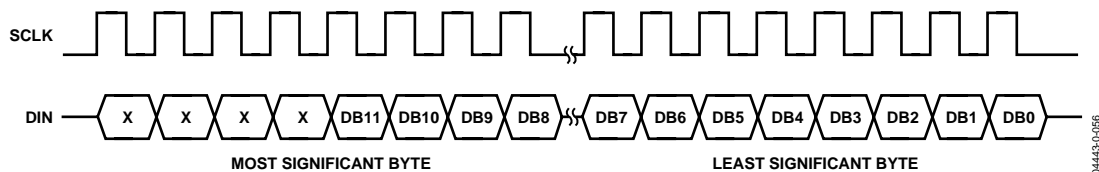
Figure 89. 12-Bit Serial Write Operation
