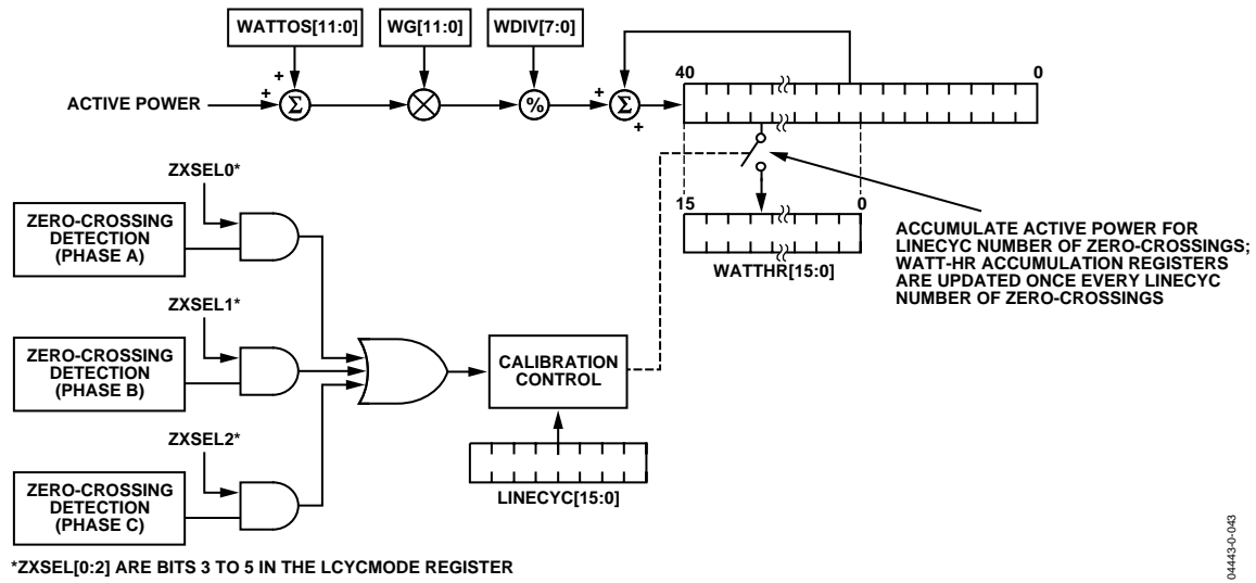
Figure 67. ADE7758 Line Cycle Active Energy Accumulation Mode
