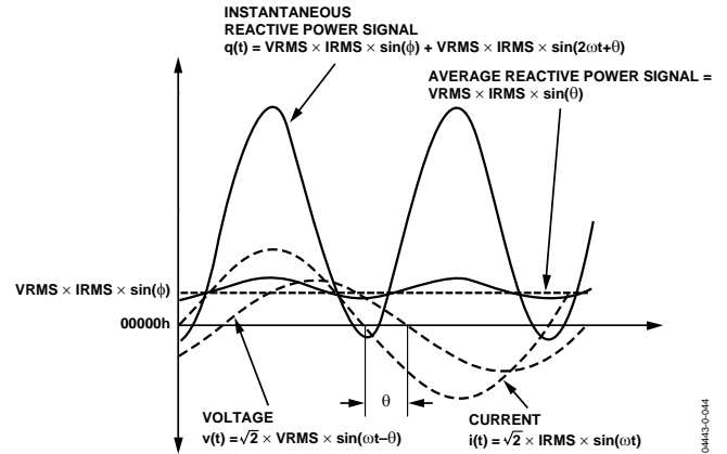
Figure 68. Reactive Power Calculation
