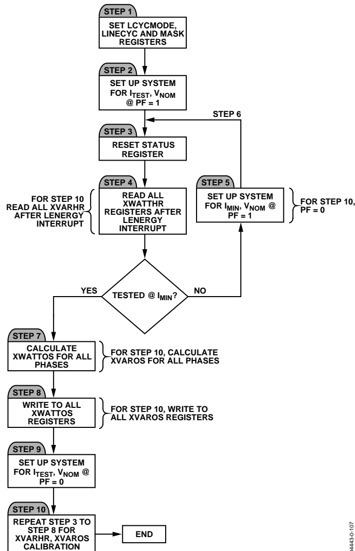
Figure 80. Power Offset Calibration Using Line Accumulation
