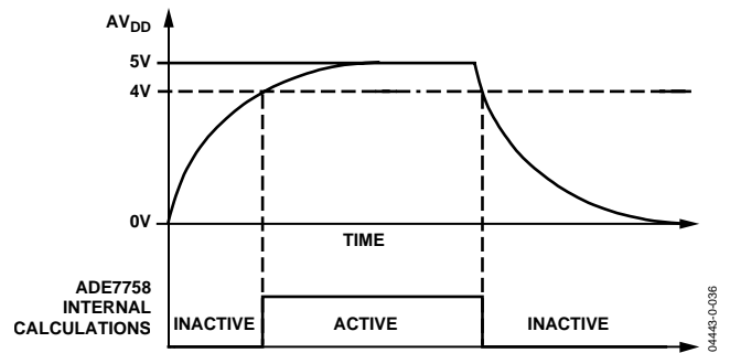
Figure 58. On-Chip Power-Supply Monitoring
