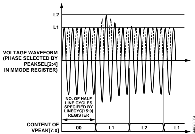
Figure 56. Peak Current Detection Using the IPEAK Register
