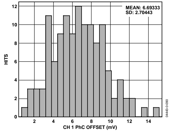
Figure 32. Phase C Channel 1 Offset Distribution
