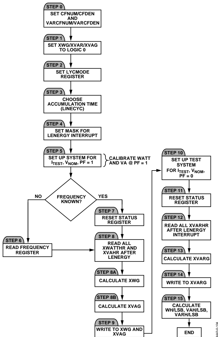
Figure 78. Gain Calibration Using Line Accumulation
