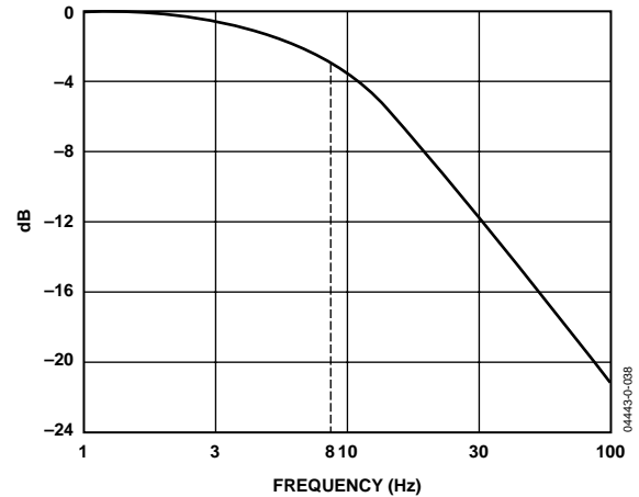
Figure 62. Frequency Response of the LPF Used to Filter Instantaneous Power in Each Phase
