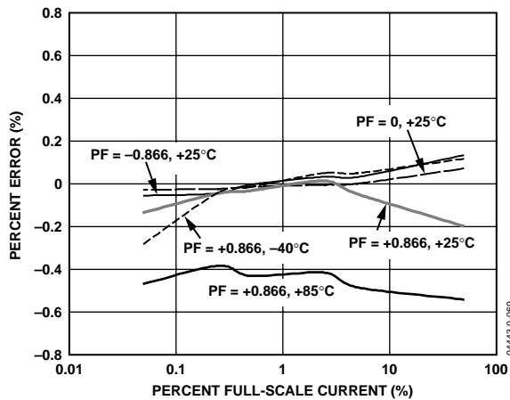
Figure 13. Reactive Energy Error as a Percentage of Reading (Gain = +1) over Power Factor with Internal Reference and Integrator Off
