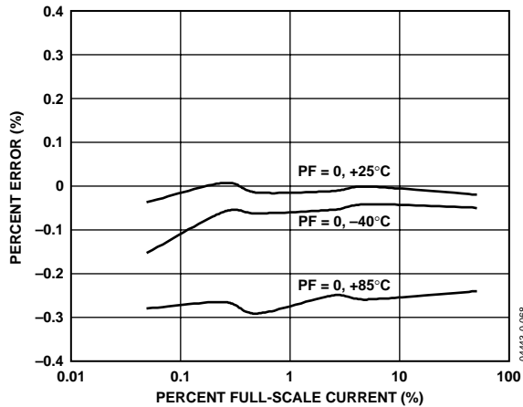
Figure 11. APCF Error as a Percentage of Reading (Gain = +1) with Internal Reference and Integrator Off
