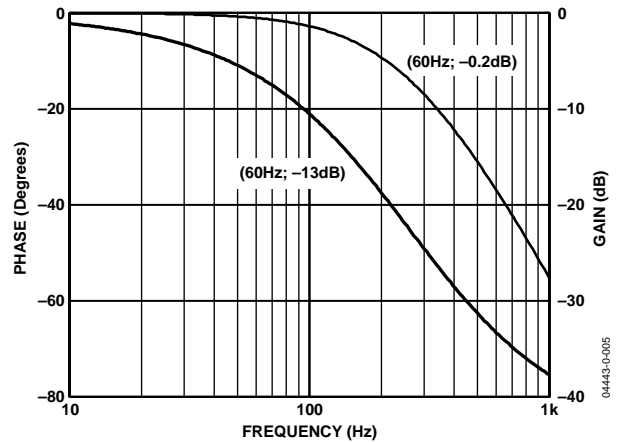
Figure 48. Magnitude and Phase Response of LPF1
