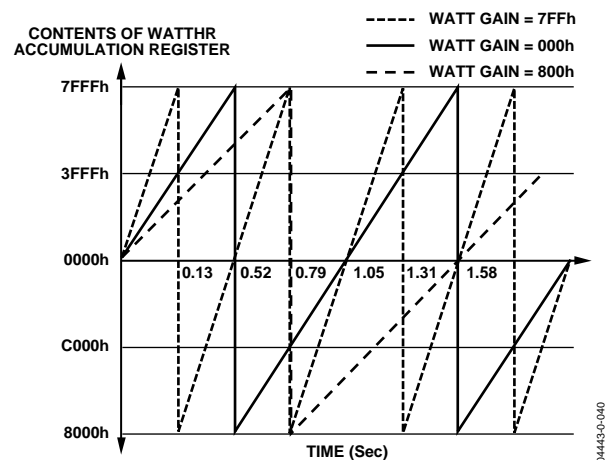
Figure 64. Energy Register Roll-Over Time for Full-Scale Power (Minimum and Maximum Power Gain)
