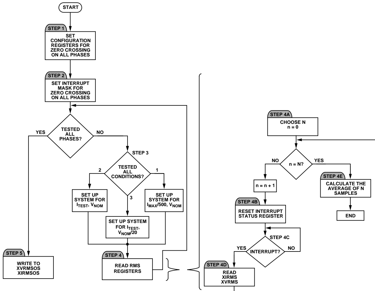
Figure 81. RMS Calibration Routine
