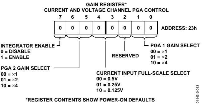
Figure 37. ADE7758 Analog Gain Register
