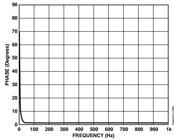
Figure 51. Phase Response of the HPF and Phase Compensation (10 Hz to 1 kHz)
