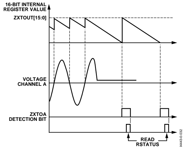
Figure 50. Zero-Crossing Timeout Detection
