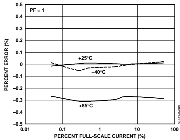
Figure 5. Active Energy Error as a Percentage of Reading (Gain = +1) over Temperature with Internal Reference and Integrator Off
