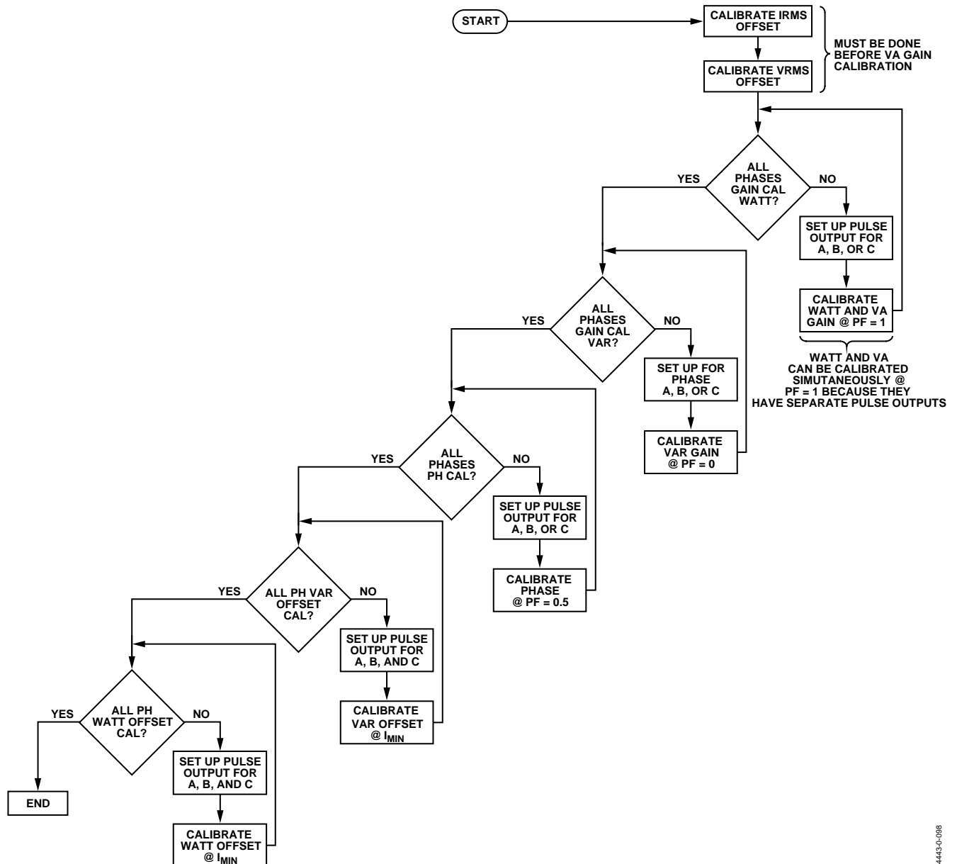
Figure 73. Calibration Using Pulse Output
