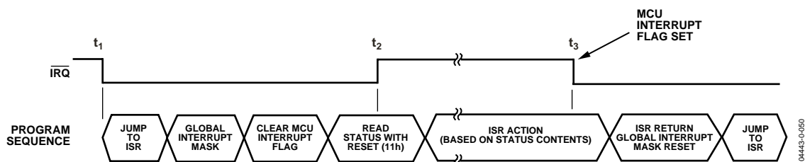
Figure 83. ADE7758 Interrupt Management
