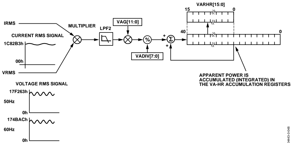
Figure 72. ADE7758 Apparent Energy Accumulation
