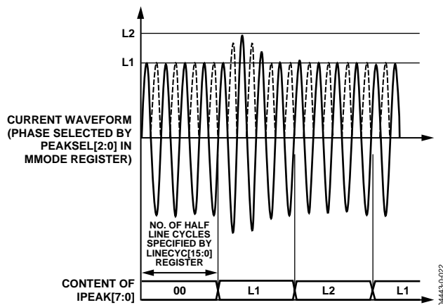
Figure 45. Peak Current Detection Using the IPEAK Register
