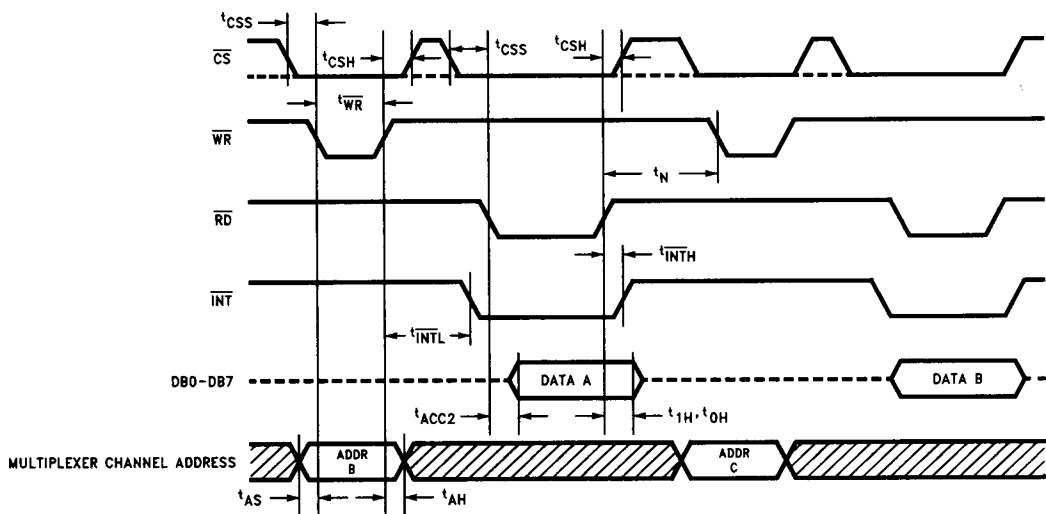
FIGURE 2b. \overline{WR} - \overline{RD} Mode (Mode Pin is High and t_{RD} > t_{INTL} )
