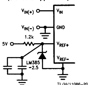
External Reference 2.5V Full-Scale (Standard Application)
