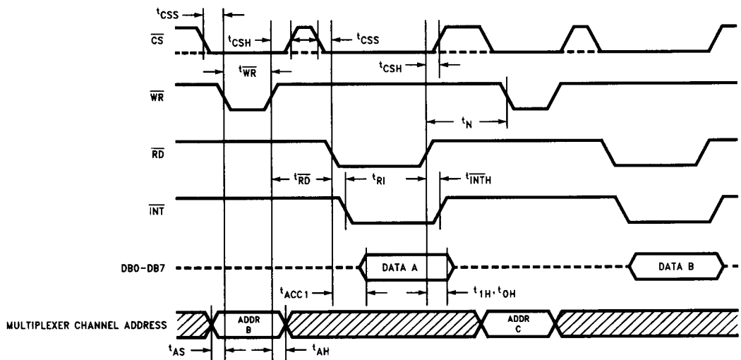
FIGURE 2a. \overline{WR} - \overline{RD} Mode (Mode Pin is High and t_{RD} \leq t_{INTL} )
