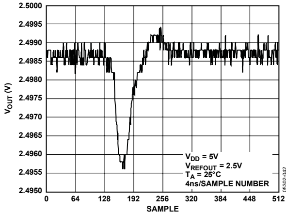
Figure 41. Analog Crosstalk
