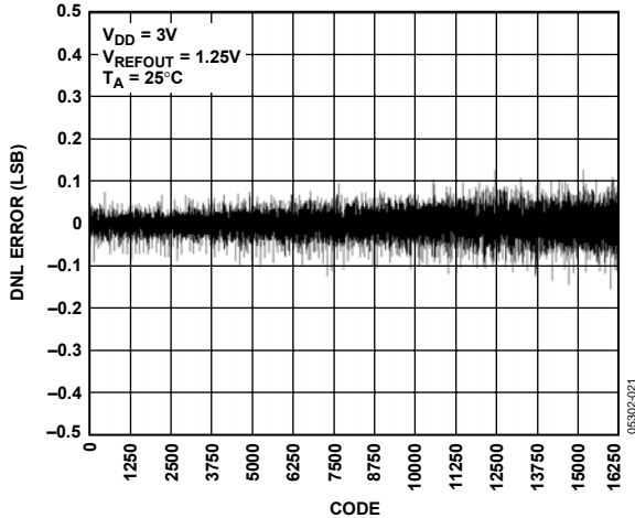
Figure 21. DNL AD5648-1
