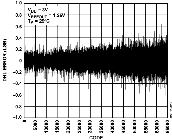
Figure 20. DNL AD5668-1
