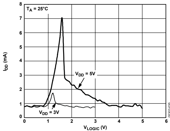
Figure 35. Supply Current vs. Logic Input Voltage
