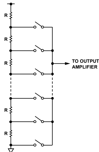
Figure 52. Resistor String
