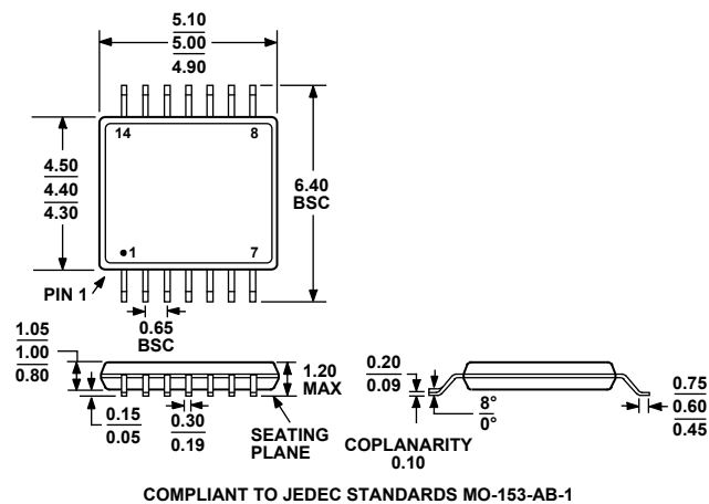
Figure 58. 14-Lead Thin Shrink Small Outline Package [TSSOP] (RU-14) Dimensions shown in millimeters
