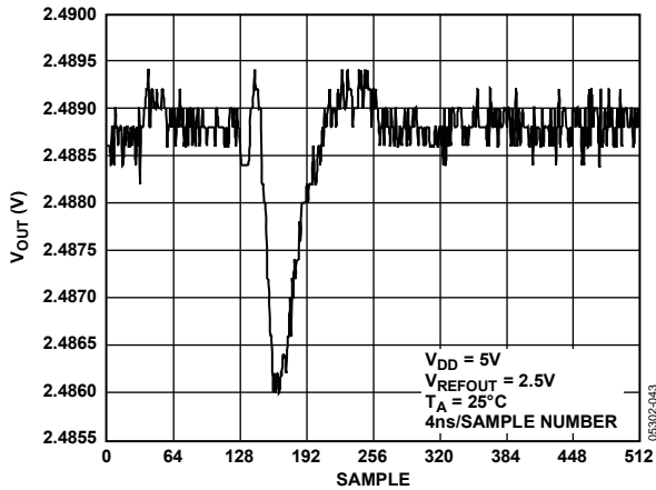
Figure 42. DAC-to-DAC Crosstalk
