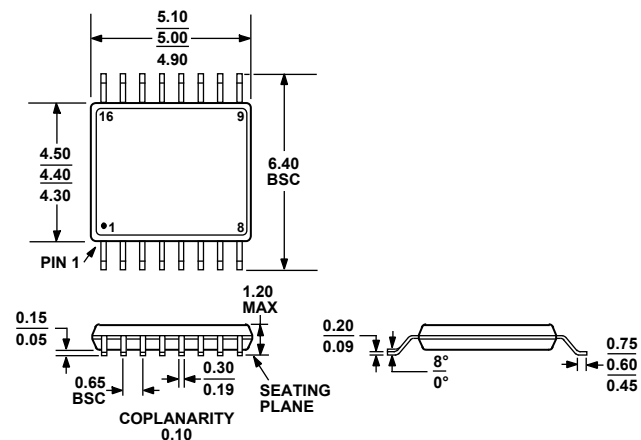
Figure 59. 16-Lead Thin Shrink Small Outline Package [TSSOP] (RU-16) Dimensions shown in millimeters
