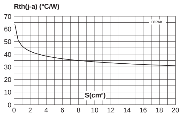
Fig. 11: Thermal resistance junction to ambient versus copper surface under tab (printed circuit board FR4, copper thickness: 35μm).
