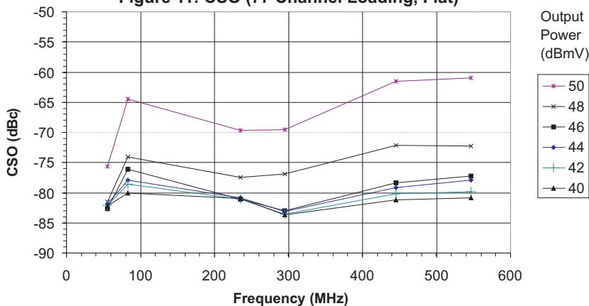
Figure 11: CSO (77 Channel Loading, Flat)
