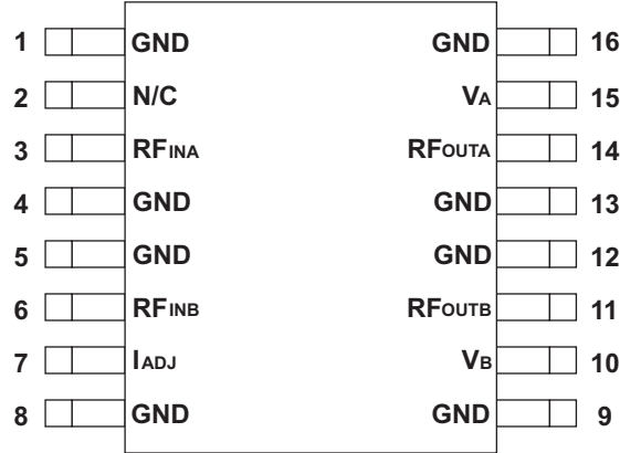
Figure 2: Pin Out
