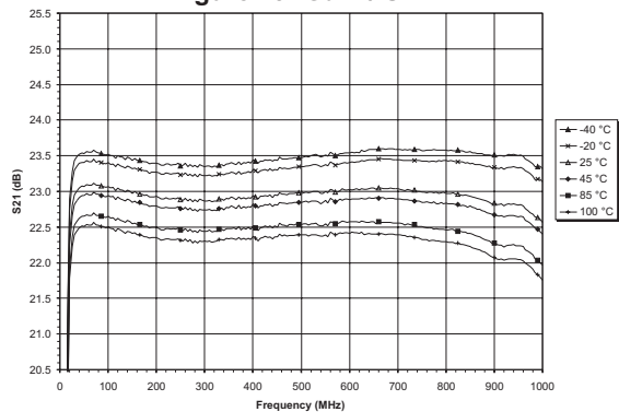
Figure 19: Gain / S21
