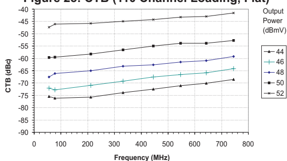
Figure 25: CTB (110 Channel Loading, Flat)
