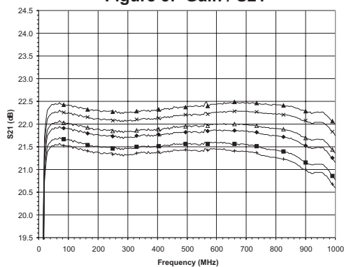
Figure 5: Gain / S21
