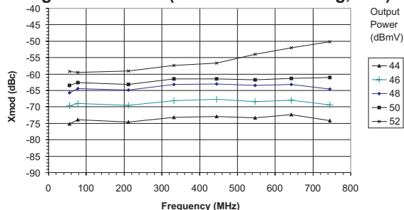
Figure 29: XMOD (110 Channel Loading, Flat)
