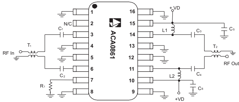
Figure 3: Test Circuit
