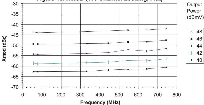
Figure 15: XMOD (110 Channel Loading, Flat)
