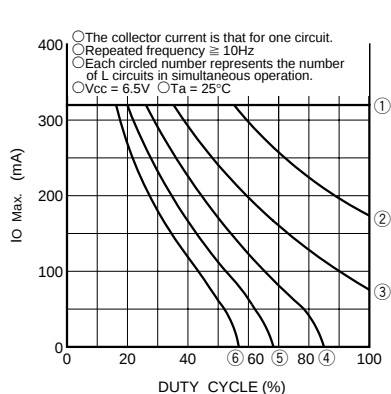
Fig. 12 Duty cycle vs. collector current ( I )
