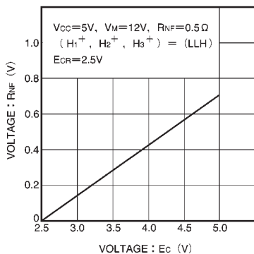
Fig.19 Output voltage vs. torque control voltage
