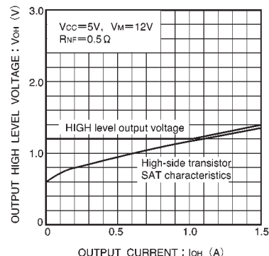
Fig.21 Output high level voltage vs. output current
