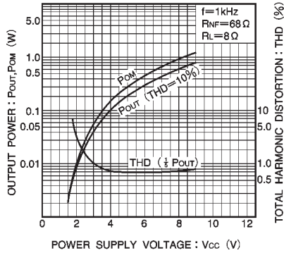
Fig. 5 Rated and max. output power and total harmonic distortion vs. power supply voltage
