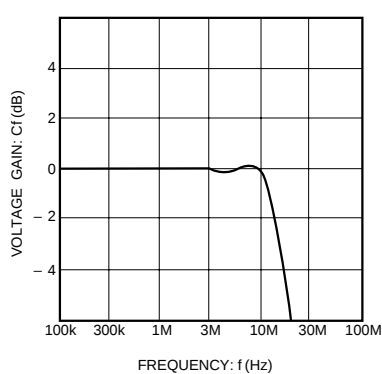
Fig. 3 Frequency characteristics
