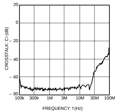
Fig. 4 Interchannel crosstalk
