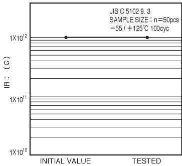
Fig.9 Insulation resistance
