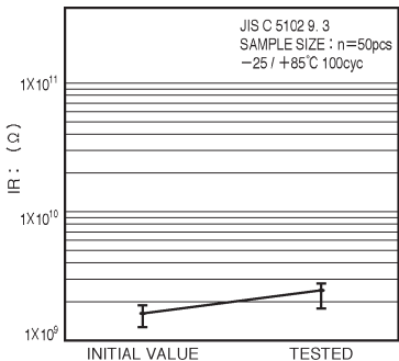
Fig.15 Insulation resistance
