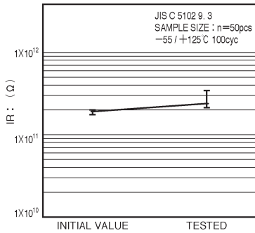
Fig.12 Insulation resistance
