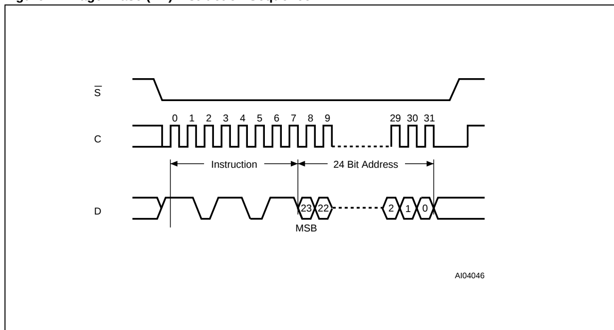
Figure 14. Page Erase (PE) Instruction Sequence
