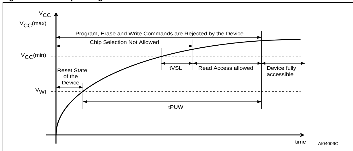
Figure 18. Power-up Timing
