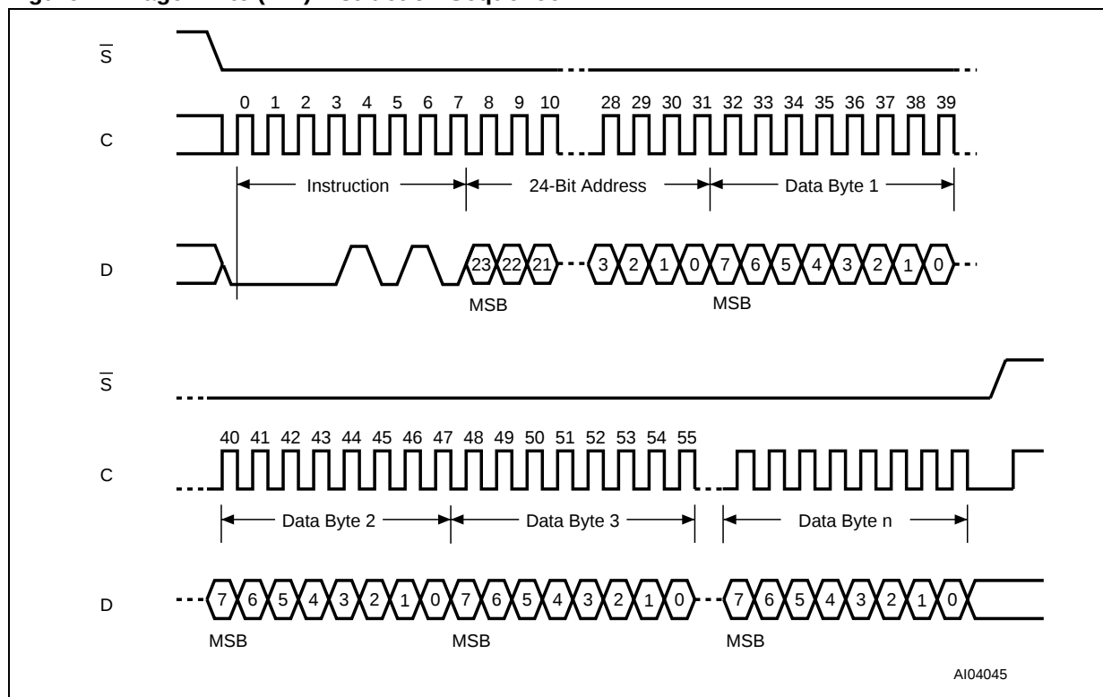
Figure 12. Page Write (PW) Instruction Sequence
