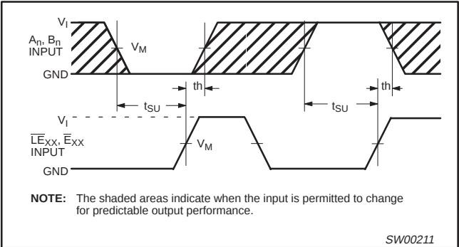
Waveform 4. Data setup and hold times for the ( A_n , B_n ) input to the \overline{LE}_{xx} and \overline{E}_{xx} inputs.
