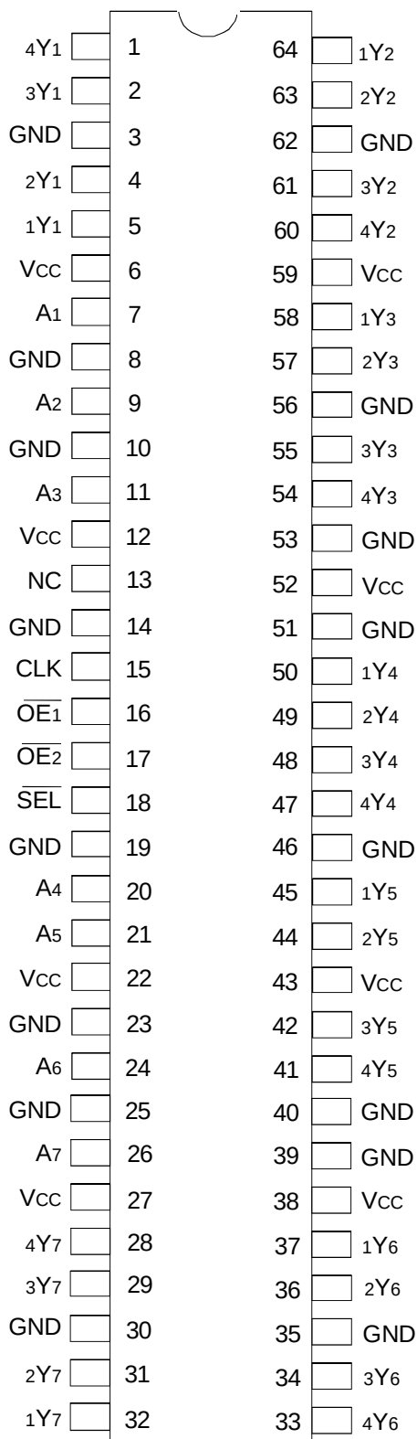
TSSOP TOP VIEW
