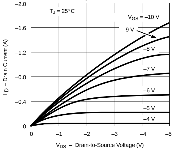
Ohmic Region Characteristics
