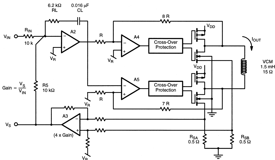
FIGURE 3. Transconductance Amplifier
