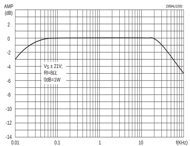
Figure 7. Frequency Response
