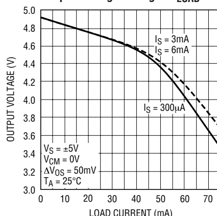
Output Voltage Swing vs I_{LO}
