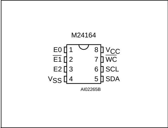
Figure 3. DIP Connections
