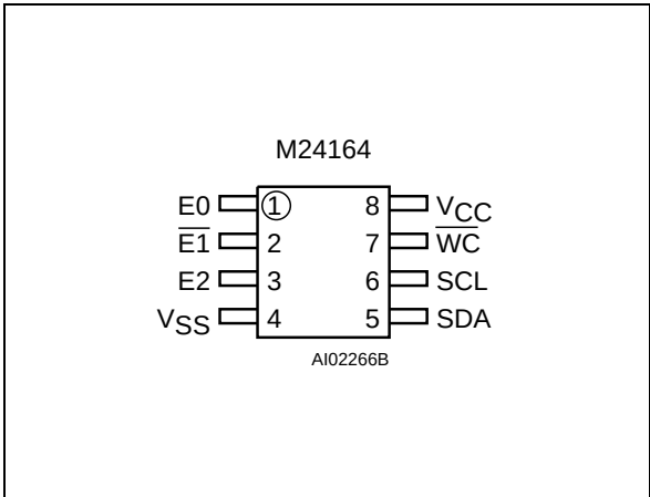
Figure 4. SO Connections
