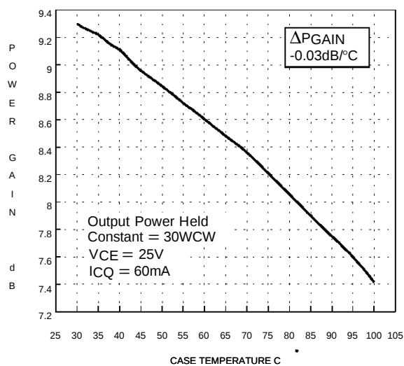
POWER GAIN vs CASE TEMPERATURE
