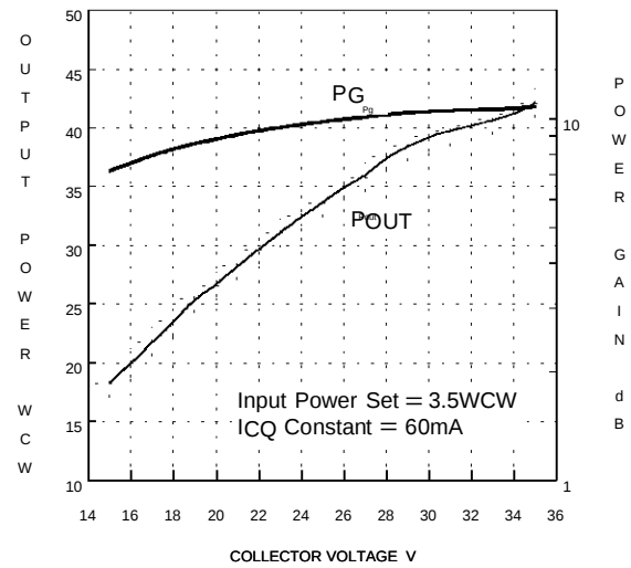
OUTPUT POWER &amp; GAIN vs VOLTAGE
