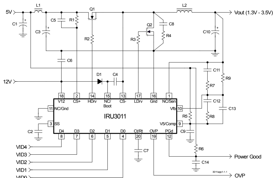
Figure 1 - Typical application of the IRU3011.
