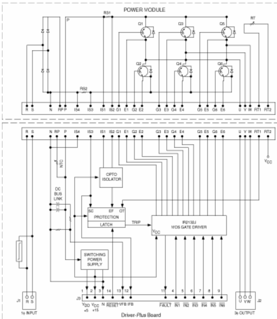
Figure 4. IRPT1058C Basic Architecture
