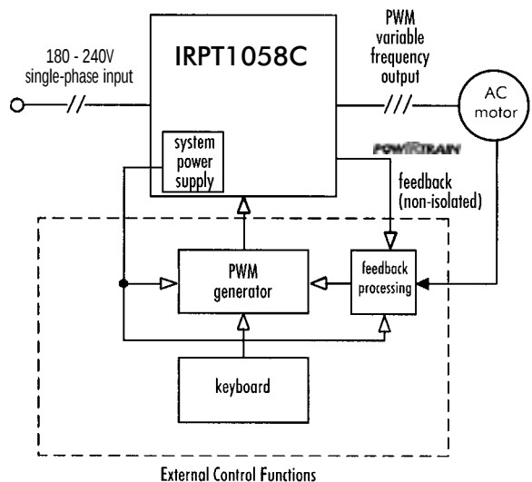
Figure 1. The IRPT1058C POWIRTRAIN within a motor control system
