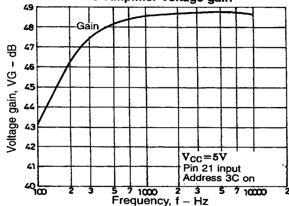
PB Amplifier voltage gain
