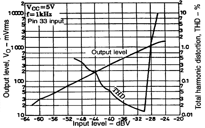
Crosspoint switch input characteristics
