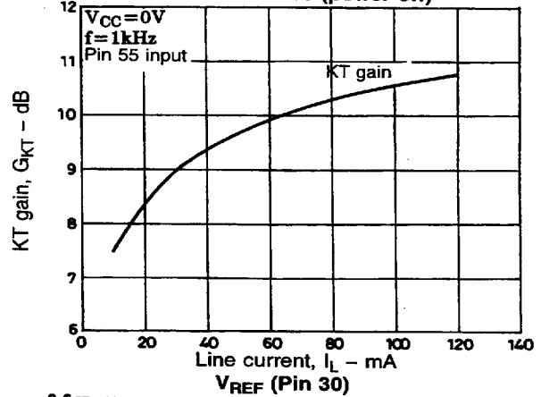
KT characteristics (power off)
