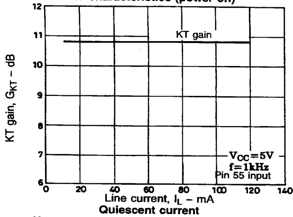
KT characteristics (power on)
