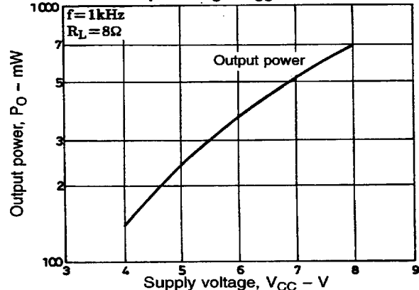
PWR Amplifier P_O - V_{CC} characteristics
