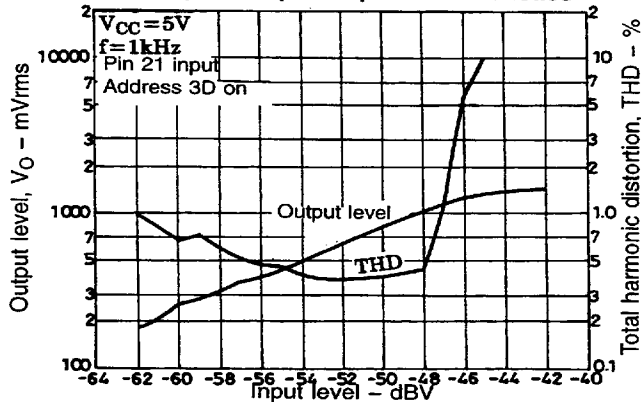
PB Amplifier input/output characteristics
