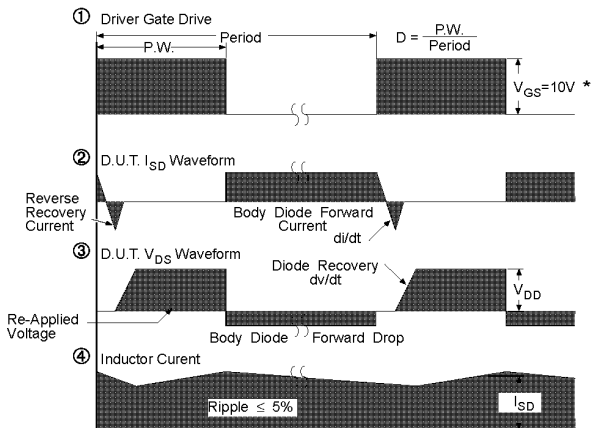
Fig 14. For N-Channel HEXFETS
