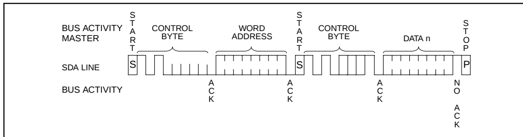
FIGURE 7-2: RANDOM READ
